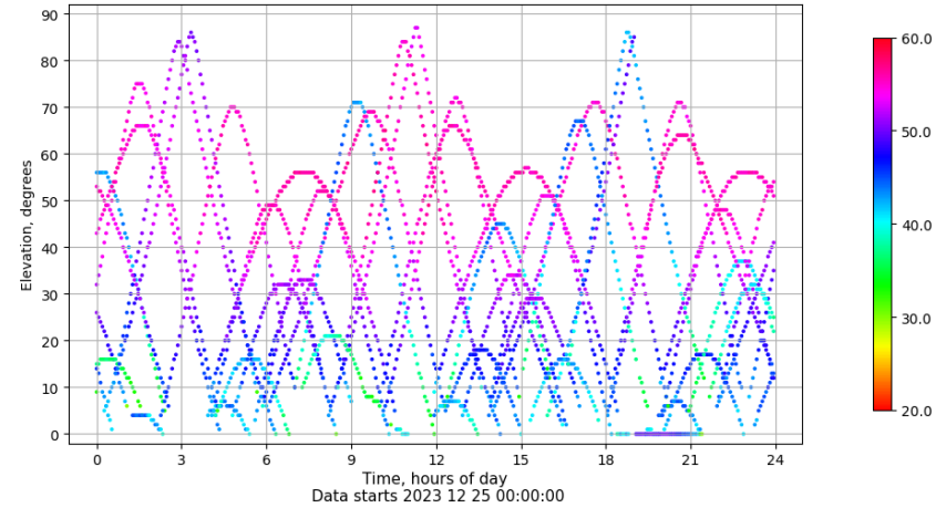
Time-elevation plot for station SPAB. Signal to Noise S1C Data file SPAB00ESP_R_2023359.xtr
