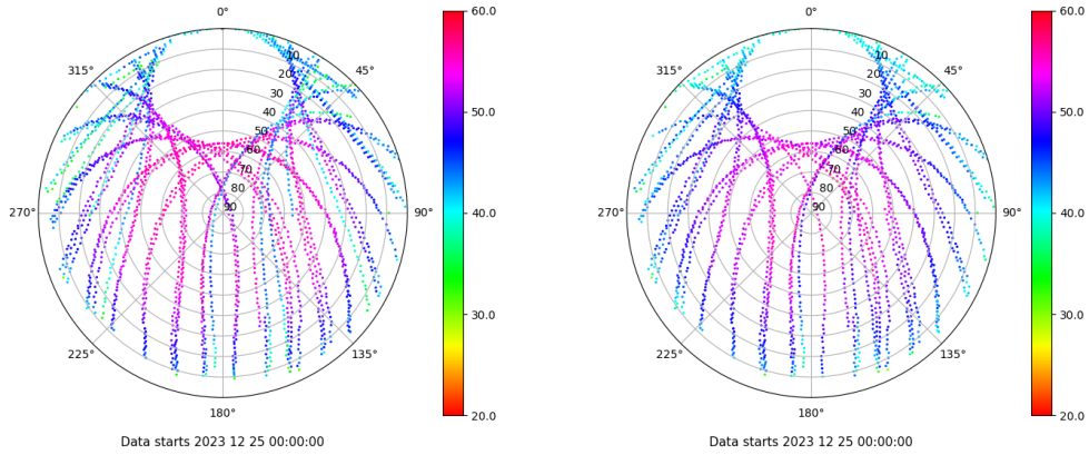
Skyplot for station SPAB. Signal to Noise S1C Data file SPAB00ESP_R_2023359.xtr Skyplot for station SPAB. Signal to Noise S2P Data file SPAB00ESP_R_2023359.xtr
