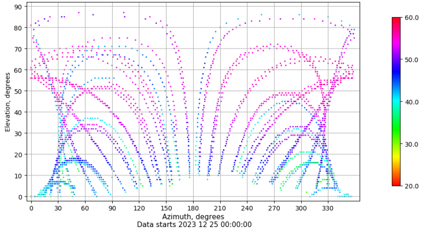
Azimuth-elevation plot for station SPAB. Signal to Noise S1C Data file SPAB00ESP_R_2023359.xtr
