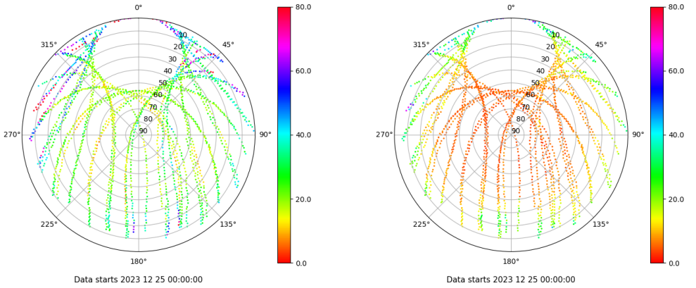
Skyplot for station SPAB. Parameter M1C Data file SPAB00ESP_R_2023359.xtr Skyplot for station SPAB. Parameter M2P Data file SPAB00ESP_R_2023359.xtr
