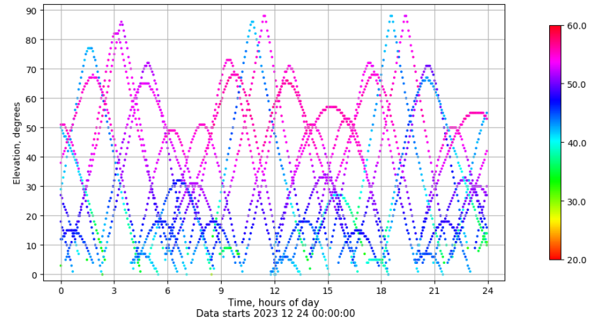
Time-elevation plot for station SPAB. Signal to Noise S1C Data file SPAB00ESP_R_2023358.xtr
