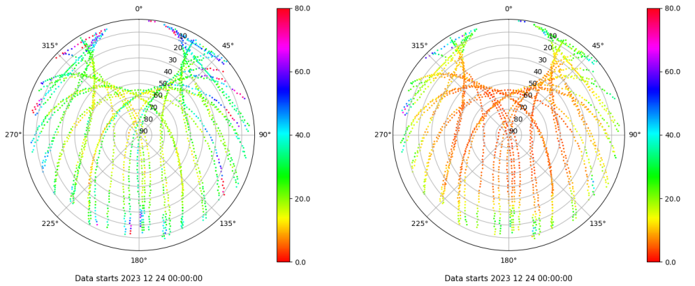
Skyplot for station SPAB. Parameter M1C Data file SPAB00ESP_R_2023358.xtr Skyplot for station SPAB. Parameter M2P Data file SPAB00ESP_R_2023358.xtr
