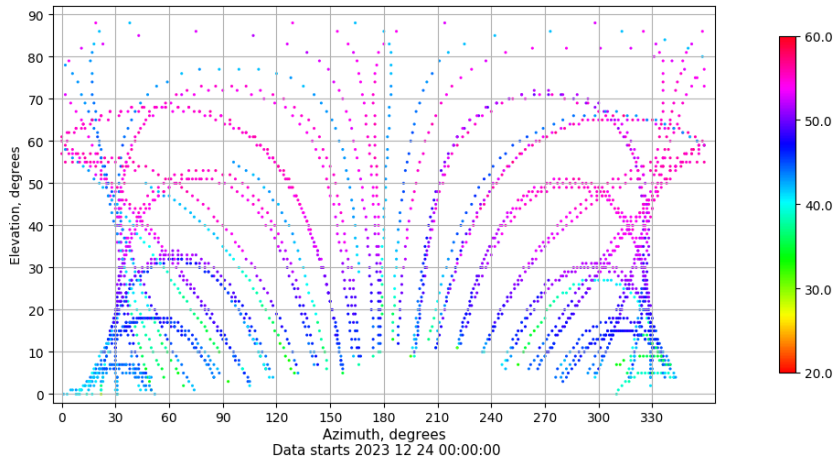
Azimuth-elevation plot for station SPAB. Signal to Noise S1C Data file SPAB00ESP_R_2023358.xtr
