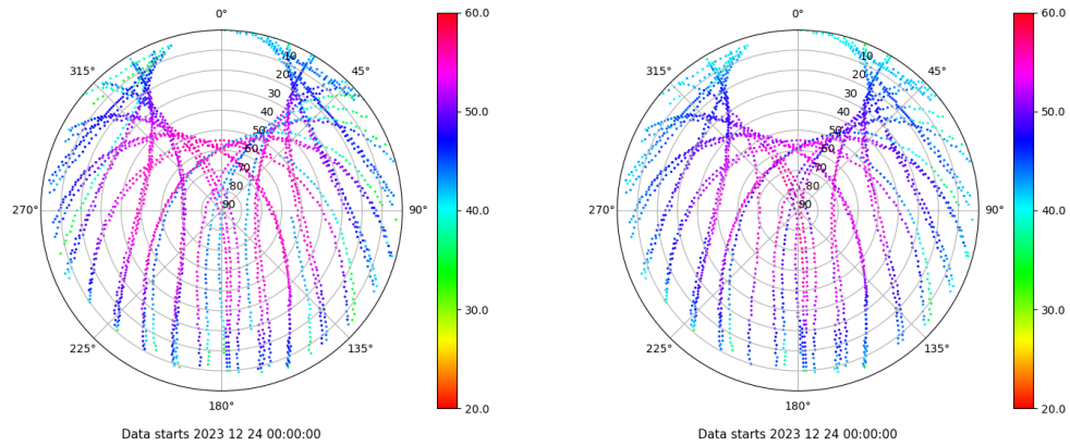
Skyplot for station SPAB. Signal to Noise S1C Data file SPAB00ESP_R_2023358.xtr Skyplot for station SPAB. Signal to Noise S2P Data file SPAB00ESP_R_2023358.xtr
