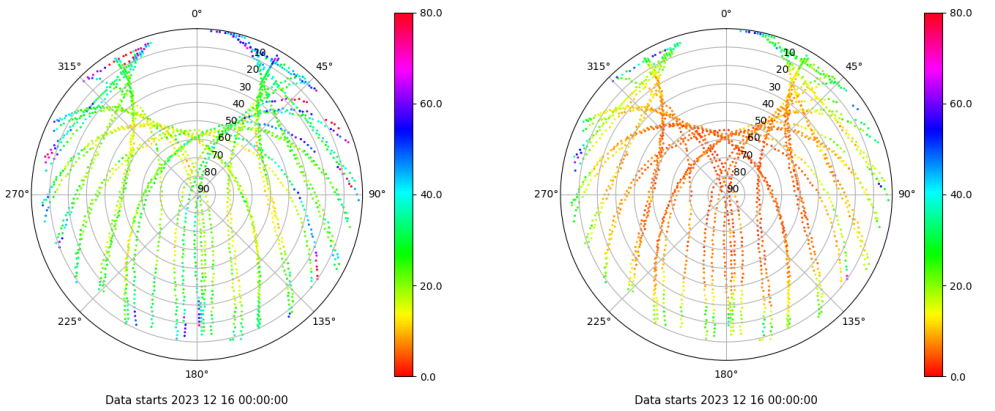
Skyplot for station SPAB. Parameter M1C Data file SPAB00ESP_R_2023350.xtr Skyplot for station SPAB. Parameter M2P Data file SPAB00ESP_R_2023350.xtr
