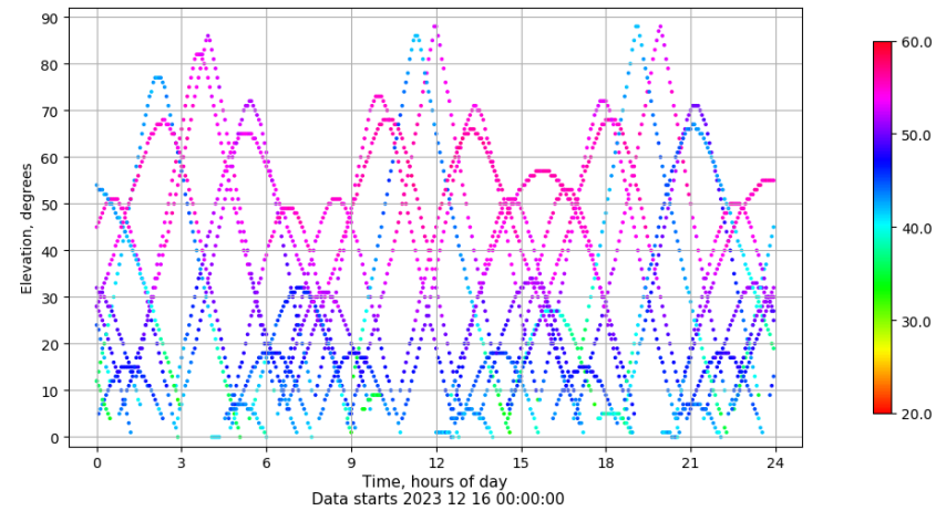
Time-elevation plot for station SPAB. Signal to Noise S1C Data file SPAB00ESP_R_2023350.xtr
