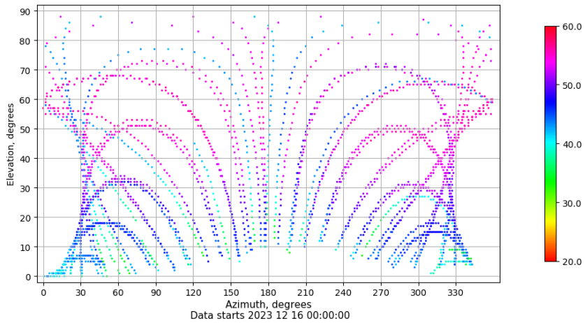
Azimuth-elevation plot for station SPAB. Signal to Noise S1C Data file SPAB00ESP_R_2023350.xtr
