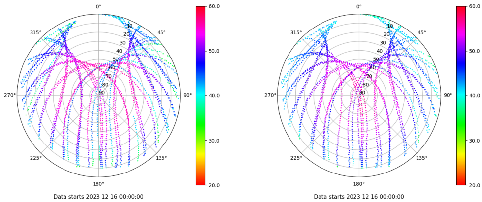
Skyplot for station SPAB. Signal to Noise S1C Data file SPAB00ESP_R_2023350.xtr Skyplot for station SPAB. Signal to Noise S2P Data file SPAB00ESP_R_2023350.xtr
