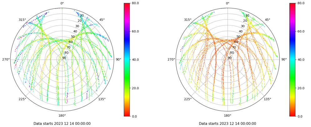
Skyplot for station SPAB. Parameter M1C Data file SPAB00ESP_R_2023348.xtr Skyplot for station SPAB. Parameter M2P Data file SPAB00ESP_R_2023348.xtr
