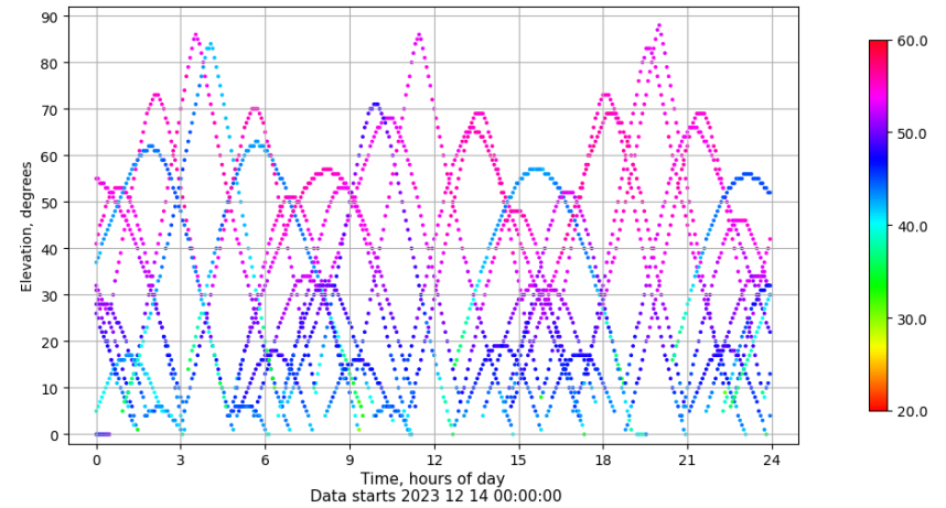
Time-elevation plot for station SPAB. Signal to Noise S1C Data file SPAB00ESP_R_2023348.xtr
