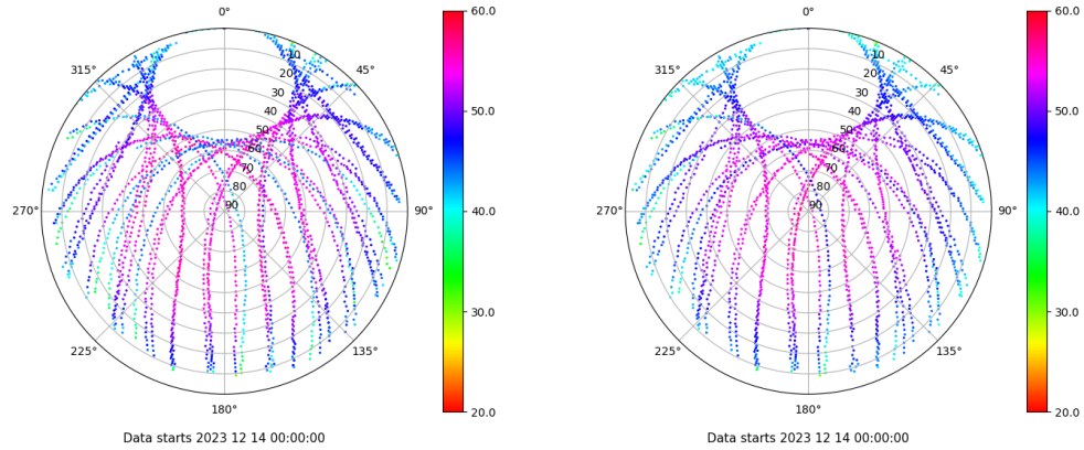
Skyplot for station SPAB. Signal to Noise S1C Data file SPAB00ESP_R_2023348.xtr Skyplot for station SPAB. Signal to Noise S2P Data file SPAB00ESP_R_2023348.xtr
