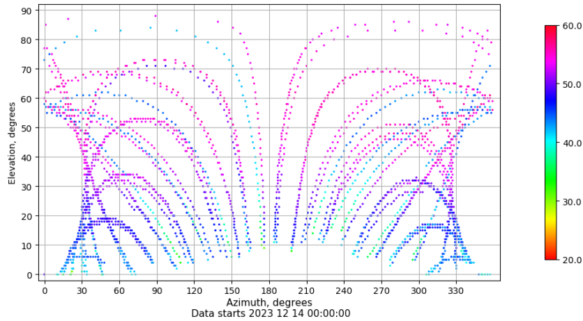
Azimuth-elevation plot for station SPAB. Signal to Noise S1C Data file SPAB00ESP_R_2023348.xtr
