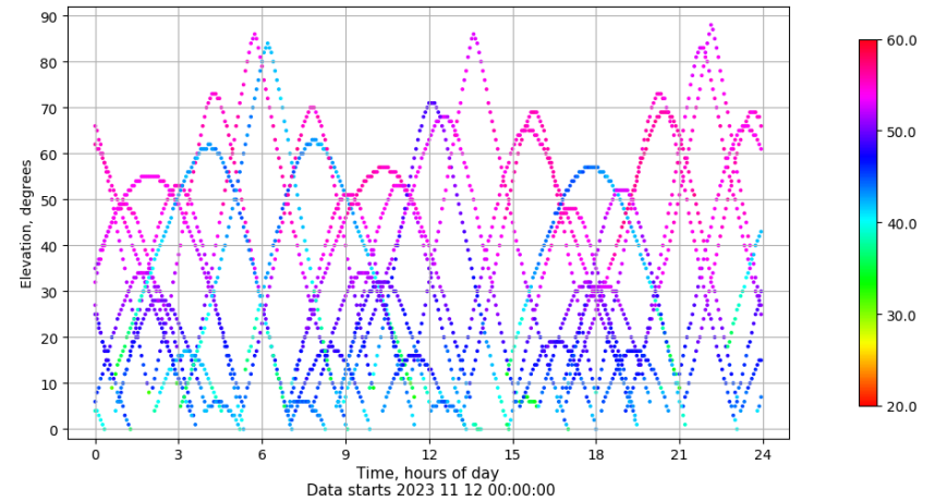
Time-elevation plot for station SPAB. Signal to Noise S1C Data file SPAB00ESP_R_2023316.xtr
