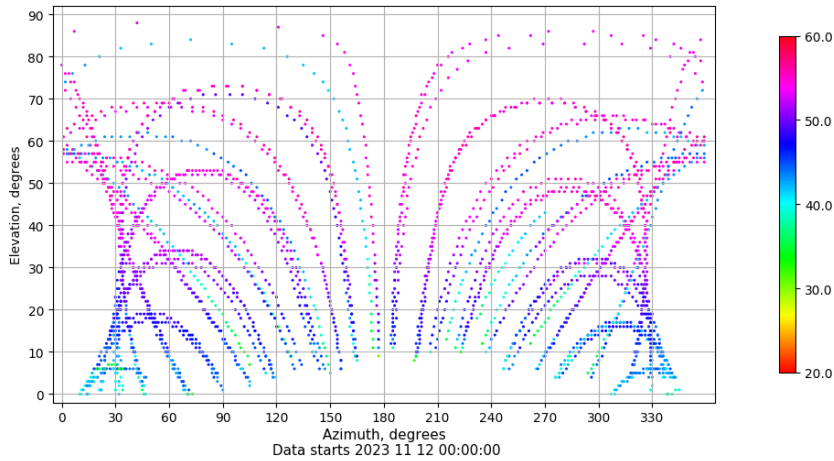
Azimuth-elevation plot for station SPAB. Signal to Noise S1C Data file SPAB00ESP_R_2023316.xtr
