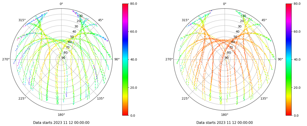
Skyplot for station SPAB. Parameter M1C Data file SPAB00ESP_R_2023316.xtr Skyplot for station SPAB. Parameter M2P Data file SPAB00ESP_R_2023316.xtr
