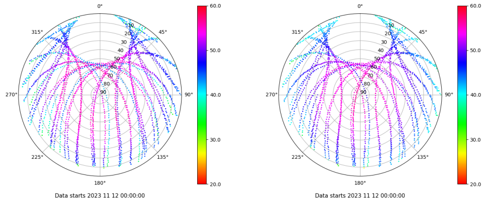
Skyplot for station SPAB. Signal to Noise S1C Data file SPAB00ESP_R_2023316.xtr Skyplot for station SPAB. Signal to Noise S2P Data file SPAB00ESP_R_2023316.xtr
