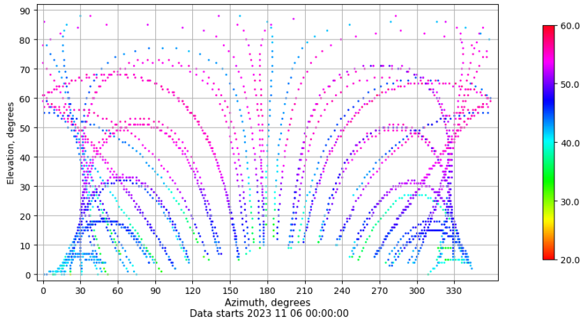
Azimuth-elevation plot for station SPAB. Signal to Noise S1C Data file SPAB00ESP_R_2023310.xtr
