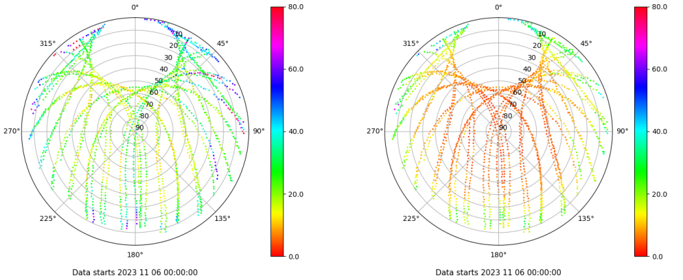
Skyplot for station SPAB. Parameter M1C Data file SPAB00ESP_R_2023310.xtr Skyplot for station SPAB. Parameter M2P Data file SPAB00ESP_R_2023310.xtr
