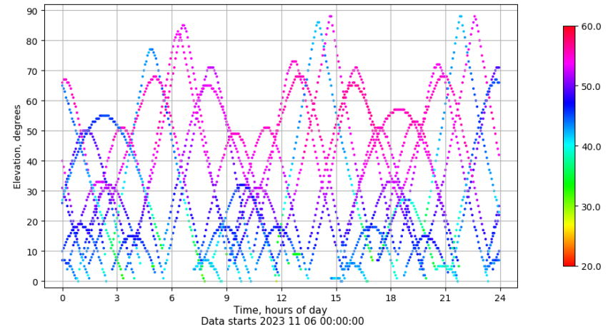
Time-elevation plot for station SPAB. Signal to Noise S1C Data file SPAB00ESP_R_2023310.xtr
