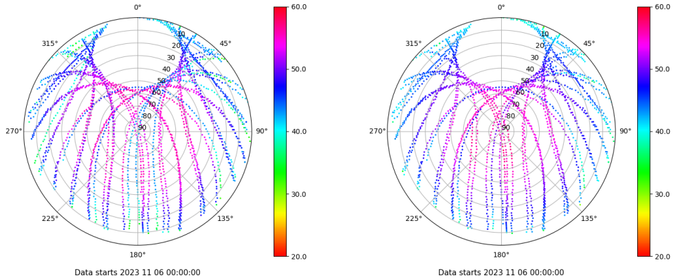
Skyplot for station SPAB. Signal to Noise S1C Data file SPAB00ESP_R_2023310.xtr Skyplot for station SPAB. Signal to Noise S2P Data file SPAB00ESP_R_2023310.xtr
