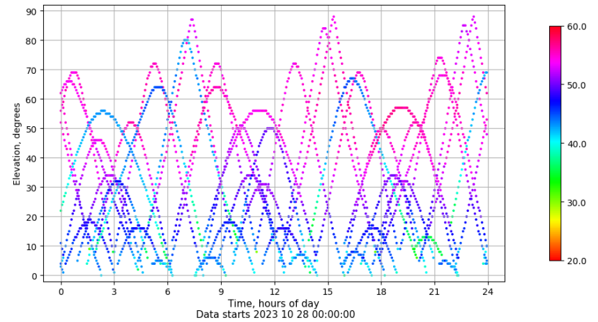
Time-elevation plot for station SPAB. Signal to Noise S1C Data file SPAB00ESP_R_2023301.xtr
