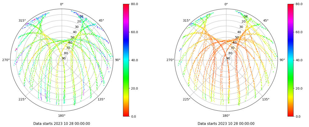
Skyplot for station SPAB. Parameter M1C Data file SPAB00ESP_R_2023301.xtr Skyplot for station SPAB. Parameter M2P Data file SPAB00ESP_R_2023301.xtr
