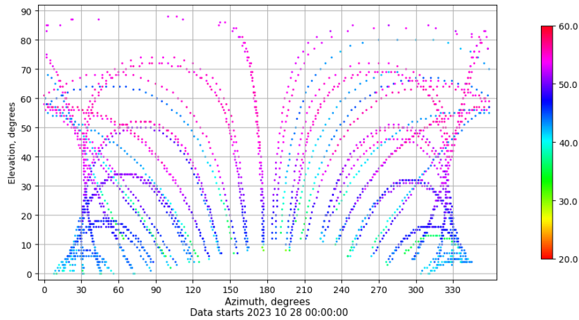
Azimuth-elevation plot for station SPAB. Signal to Noise S1C Data file SPAB00ESP_R_2023301.xtr
