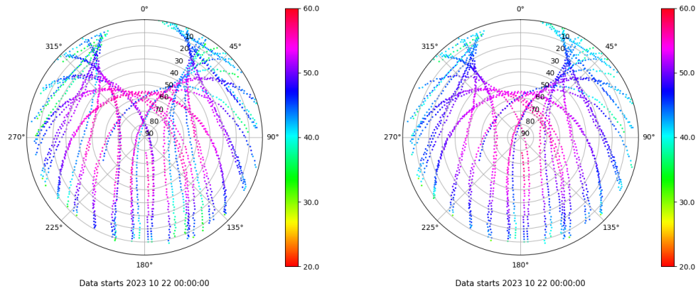
Skyplot for station SPAB. Signal to Noise S1C Data file SPAB00ESP_R_2023295.xtr Skyplot for station SPAB. Signal to Noise S2P Data file SPAB00ESP_R_2023295.xtr
