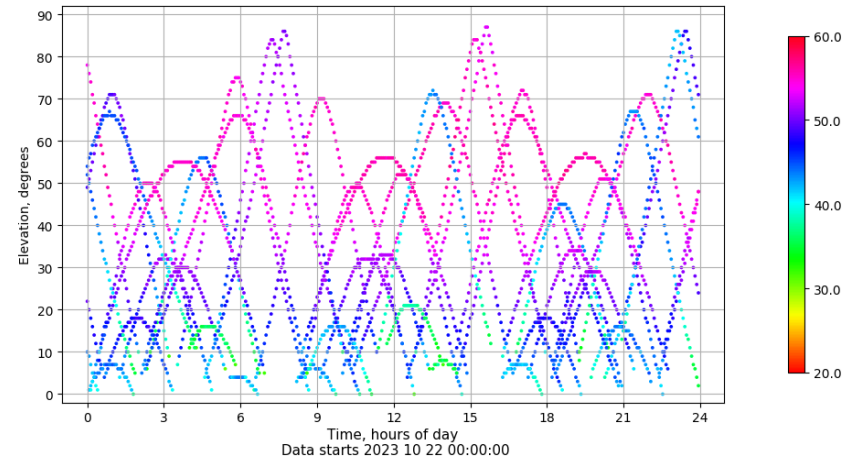
Time-elevation plot for station SPAB. Signal to Noise S1C Data file SPAB00ESP_R_2023295.xtr
