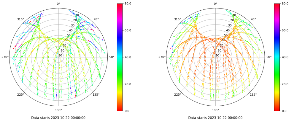
Skyplot for station SPAB. Parameter M1C Data file SPAB00ESP_R_2023295.xtr Skyplot for station SPAB. Parameter M2P Data file SPAB00ESP_R_2023295.xtr
