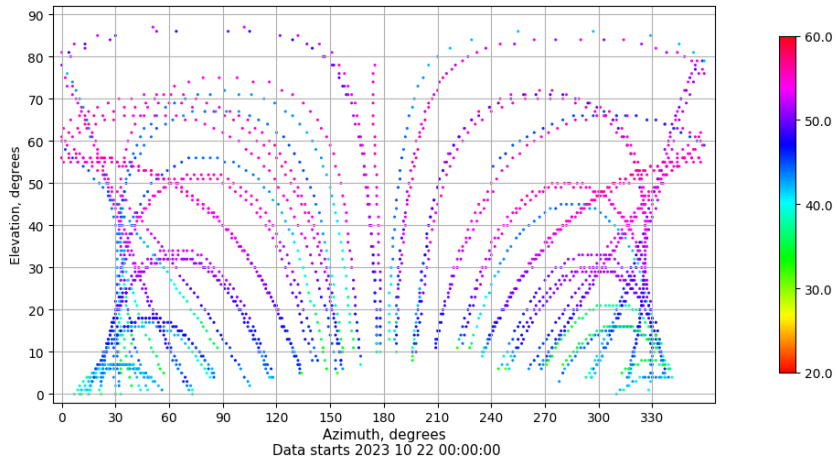
Azimuth-elevation plot for station SPAB. Signal to Noise S1C Data file SPAB00ESP_R_2023295.xtr
