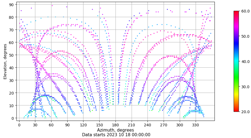
Azimuth-elevation plot for station SPAB. Signal to Noise S1C Data file SPAB00ESP_R_2023291.xtr
