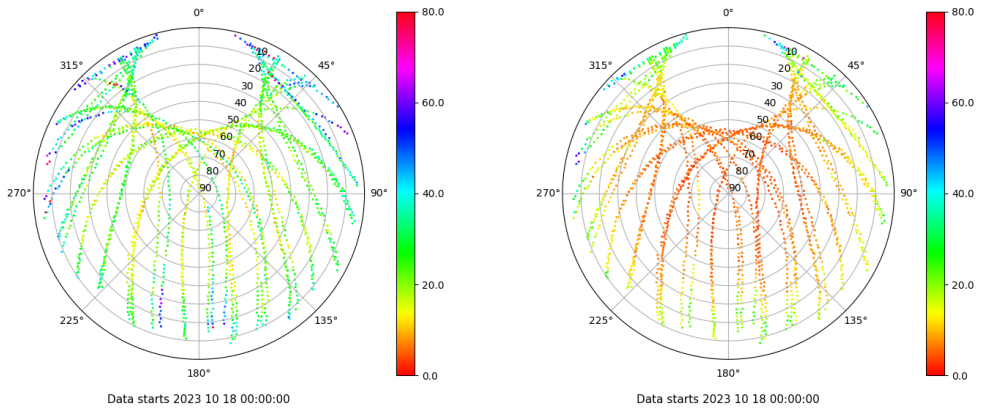
Skyplot for station SPAB. Parameter M1C Data file SPAB00ESP_R_2023291.xtr Skyplot for station SPAB. Parameter M2P Data file SPAB00ESP_R_2023291.xtr
