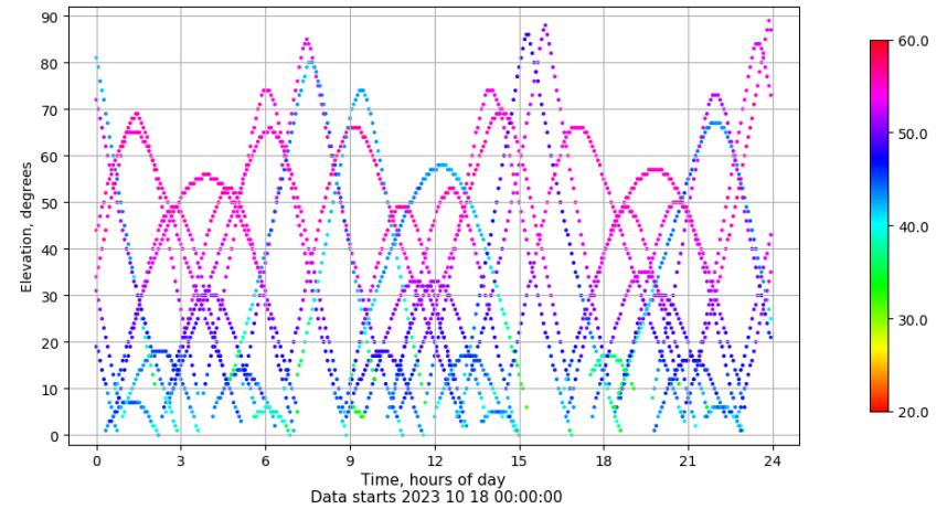
Time-elevation plot for station SPAB. Signal to Noise S1C Data file SPAB00ESP_R_2023291.xtr
