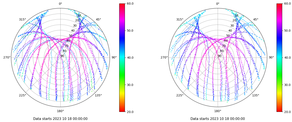
Skyplot for station SPAB. Signal to Noise S1C Data file SPAB00ESP_R_2023291.xtr Skyplot for station SPAB. Signal to Noise S2P Data file SPAB00ESP_R_2023291.xtr
