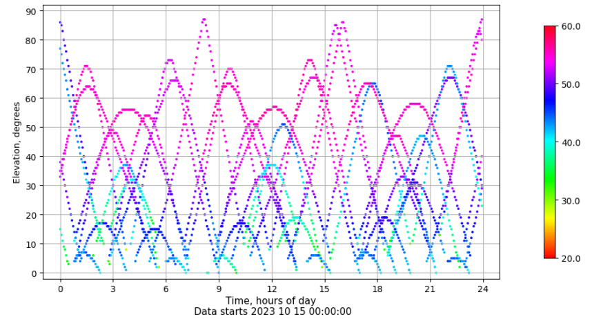
Time-elevation plot for station SPAB. Signal to Noise S1C Data file SPAB00ESP_R_2023288.xtr
