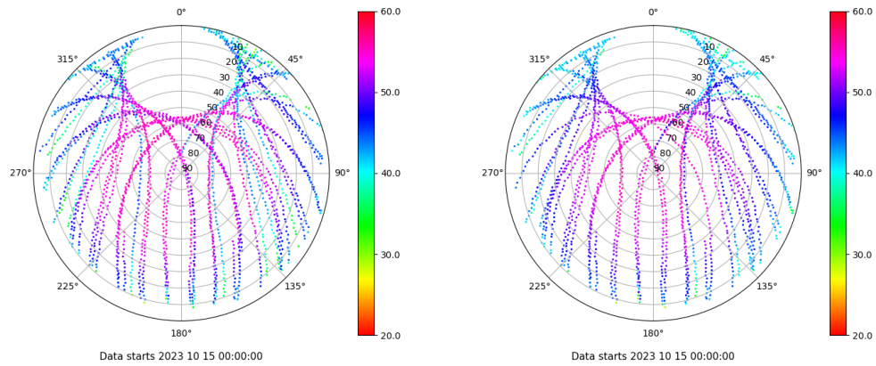
Skyplot for station SPAB. Signal to Noise S1C Data file SPAB00ESP_R_2023288.xtr Skyplot for station SPAB. Signal to Noise S2P Data file SPAB00ESP_R_2023288.xtr
