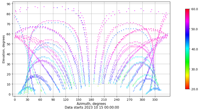
Azimuth-elevation plot for station SPAB. Signal to Noise S1C Data file SPAB00ESP_R_2023288.xtr
