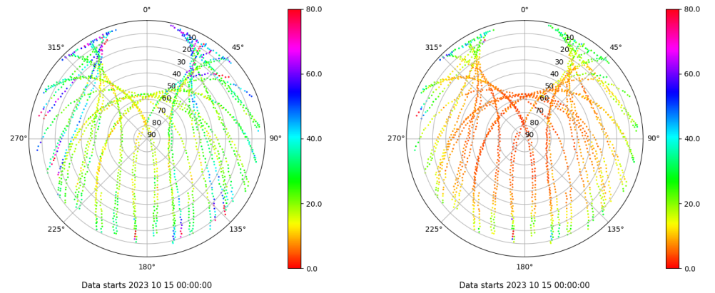
Skyplot for station SPAB. Parameter M1C Data file SPAB00ESP_R_2023288.xtr Skyplot for station SPAB. Parameter M2P Data file SPAB00ESP_R_2023288.xtr
