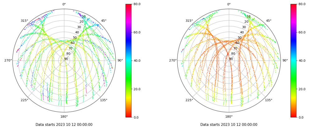
Skyplot for station SPAB. Parameter M1C Data file SPAB00ESP_R_2023285.xtr Skyplot for station SPAB. Parameter M2P Data file SPAB00ESP_R_2023285.xtr
