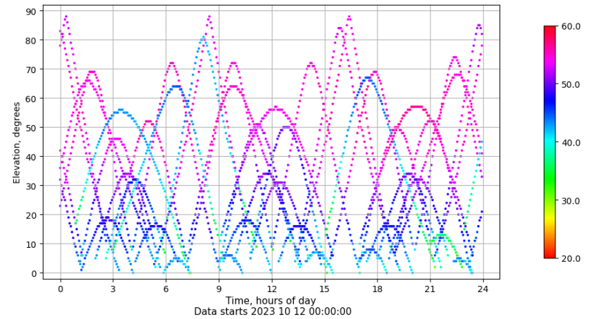
Time-elevation plot for station SPAB. Signal to Noise S1C Data file SPAB00ESP_R_2023285.xtr
