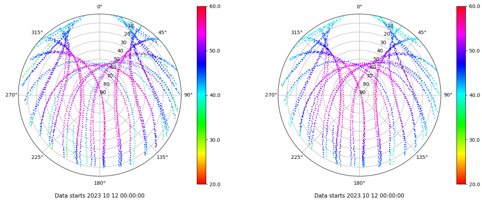
Skyplot for station SPAB. Signal to Noise S1C Data file SPAB00ESP_R_2023285.xtr Skyplot for station SPAB. Signal to Noise S2P Data file SPAB00ESP_R_2023285.xtr
