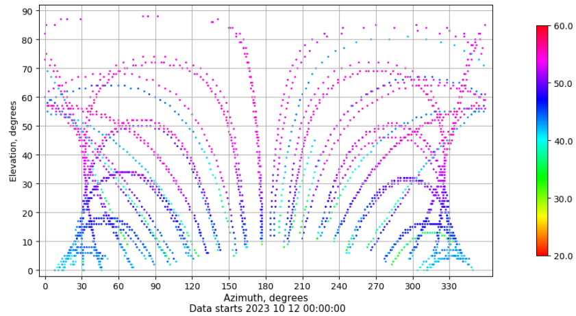
Azimuth-elevation plot for station SPAB. Signal to Noise S1C Data file SPAB00ESP_R_2023285.xtr
