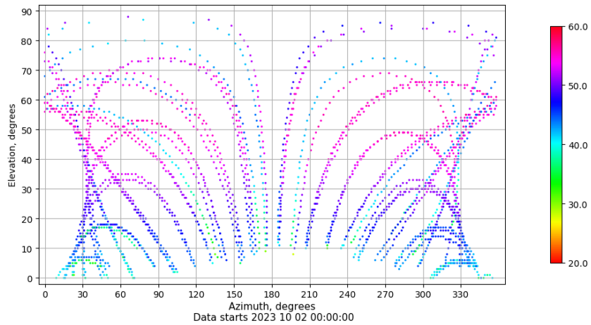
Azimuth-elevation plot for station SPAB. Signal to Noise S1C Data file SPAB00ESP_R_2023275.xtr
