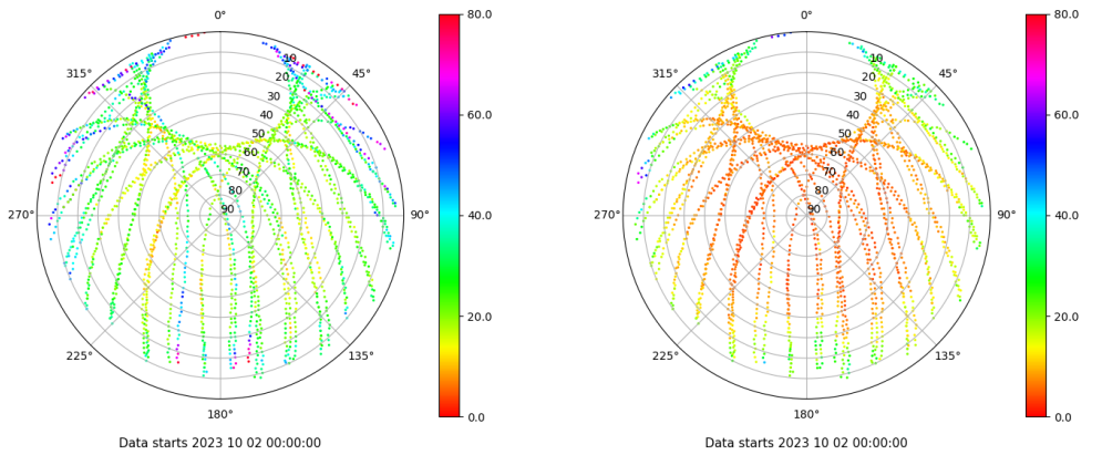
Skyplot for station SPAB. Parameter M1C Data file SPAB00ESP_R_2023275.xtr Skyplot for station SPAB. Parameter M2P Data file SPAB00ESP_R_2023275.xtr
