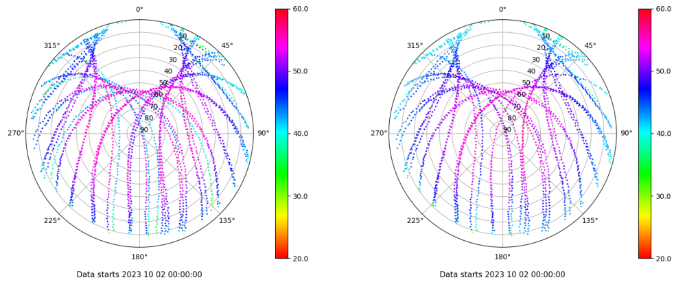
Skyplot for station SPAB. Signal to Noise S1C Data file SPAB00ESP_R_2023275.xtr Skyplot for station SPAB. Signal to Noise S2P Data file SPAB00ESP_R_2023275.xtr
