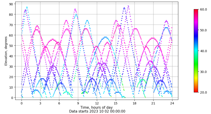
Time-elevation plot for station SPAB. Signal to Noise S1C Data file SPAB00ESP_R_2023275.xtr
