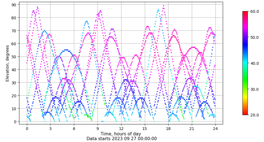
Time-elevation plot for station SPAB. Signal to Noise S1C Data file SPAB00ESP_R_2023270.xtr
