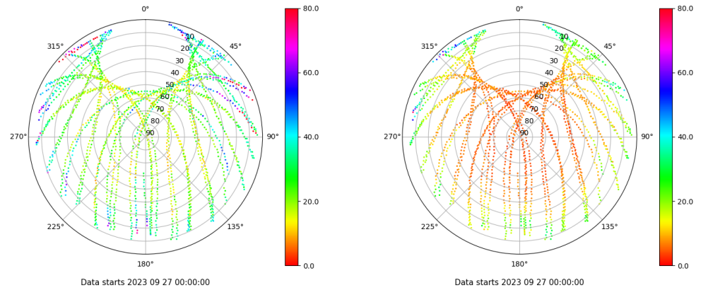
Skyplot for station SPAB. Parameter M1C Data file SPAB00ESP_R_2023270.xtr Skyplot for station SPAB. Parameter M2P Data file SPAB00ESP_R_2023270.xtr
