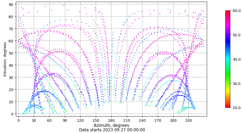
Azimuth-elevation plot for station SPAB. Signal to Noise S1C Data file SPAB00ESP_R_2023270.xtr
