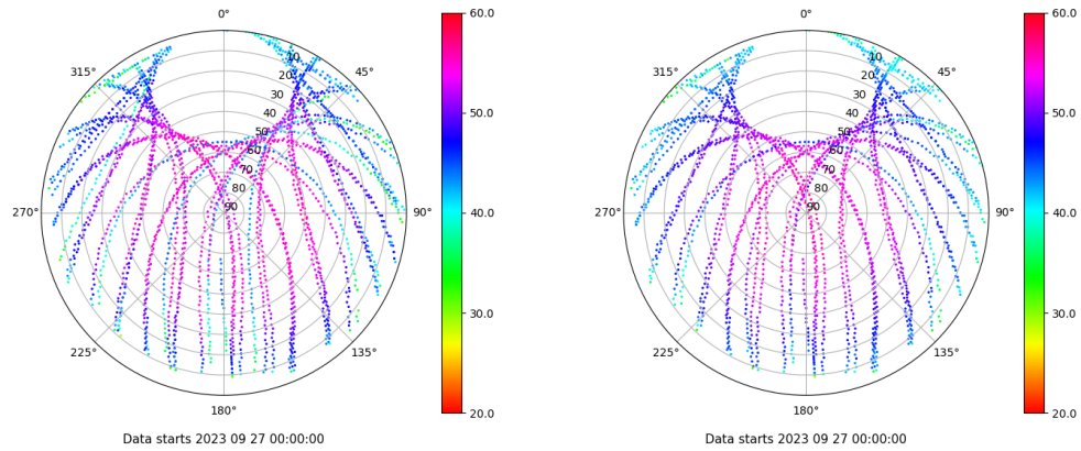
Skyplot for station SPAB. Signal to Noise S1C Data file SPAB00ESP_R_2023270.xtr Skyplot for station SPAB. Signal to Noise S2P Data file SPAB00ESP_R_2023270.xtr
