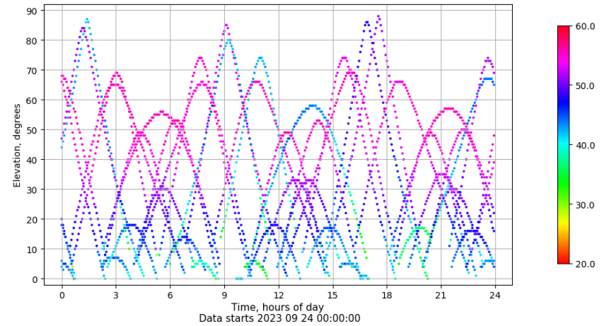
Time-elevation plot for station SPAB. Signal to Noise S1C Data file SPAB00ESP_R_2023267.xtr
