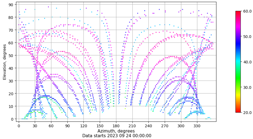
Azimuth-elevation plot for station SPAB. Signal to Noise S1C Data file SPAB00ESP_R_2023267.xtr
