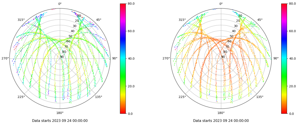
Skyplot for station SPAB. Parameter M1C Data file SPAB00ESP_R_2023267.xtr Skyplot for station SPAB. Parameter M2P Data file SPAB00ESP_R_2023267.xtr
