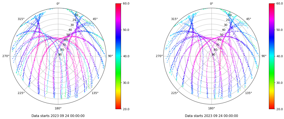
Skyplot for station SPAB. Signal to Noise S1C Data file SPAB00ESP_R_2023267.xtr Skyplot for station SPAB. Signal to Noise S2P Data file SPAB00ESP_R_2023267.xtr
