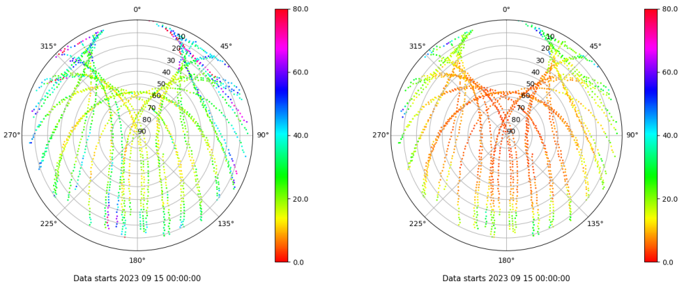
Skyplot for station SPAB. Parameter M1C Data file SPAB00ESP_R_2023258.xtr Skyplot for station SPAB. Parameter M2P Data file SPAB00ESP_R_2023258.xtr
