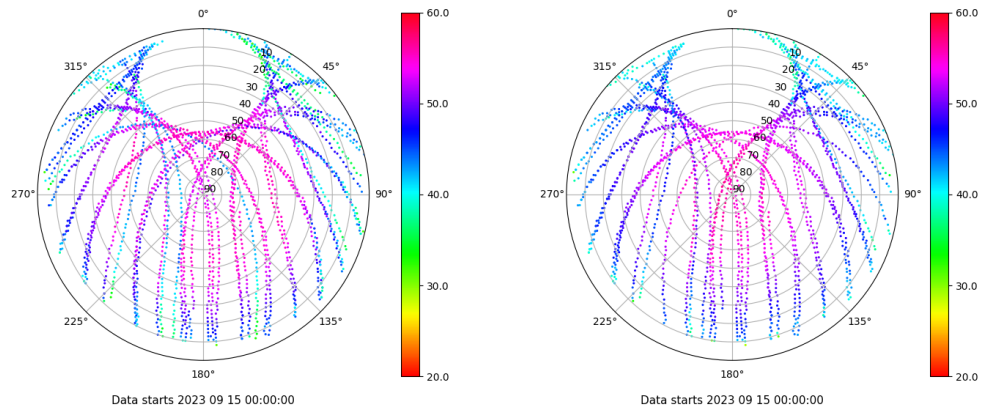
Skyplot for station SPAB. Signal to Noise S1C Data file SPAB00ESP_R_2023258.xtr Skyplot for station SPAB. Signal to Noise S2P Data file SPAB00ESP_R_2023258.xtr
