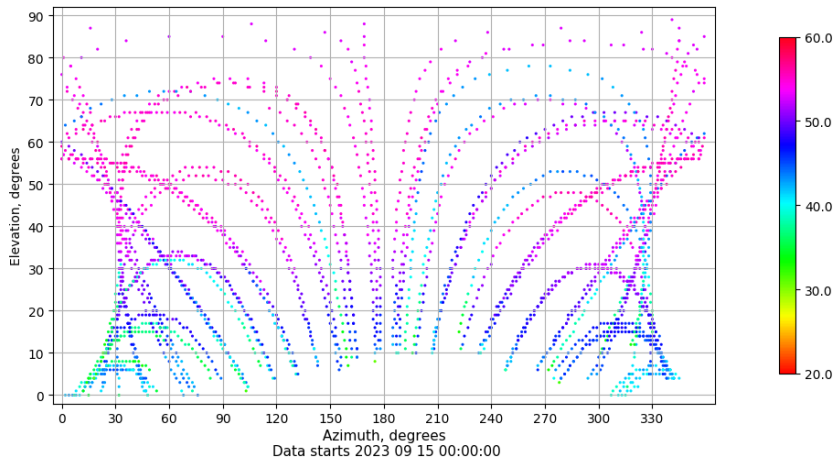
Azimuth-elevation plot for station SPAB. Signal to Noise S1C Data file SPAB00ESP_R_2023258.xtr
