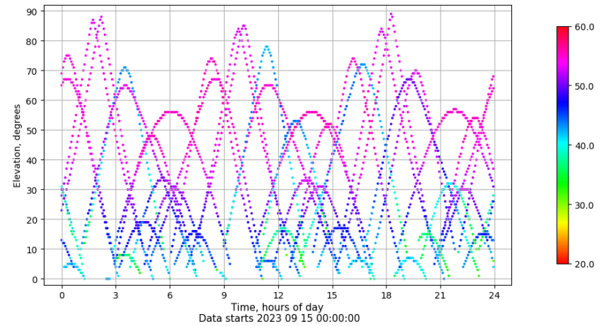
Time-elevation plot for station SPAB. Signal to Noise S1C Data file SPAB00ESP_R_2023258.xtr
