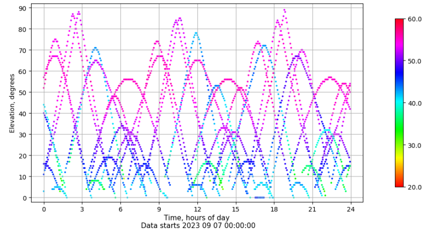
Time-elevation plot for station SPAB. Signal to Noise S1C Data file SPAB00ESP_R_2023250.xtr
