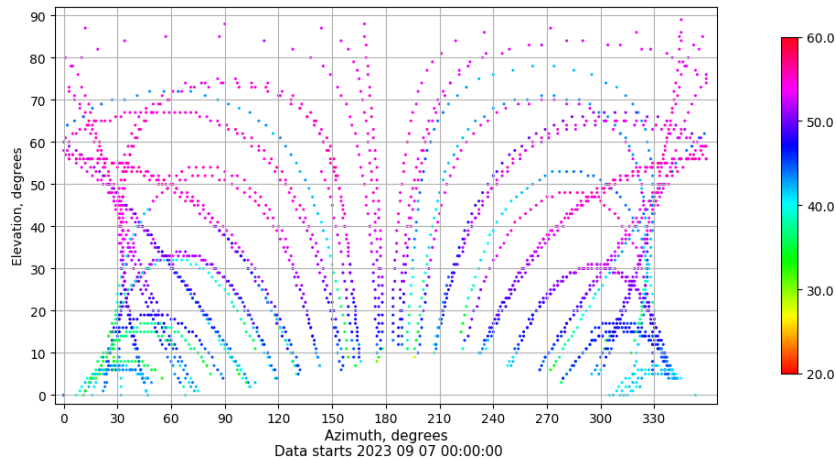
Azimuth-elevation plot for station SPAB. Signal to Noise S1C Data file SPAB00ESP_R_2023250.xtr
