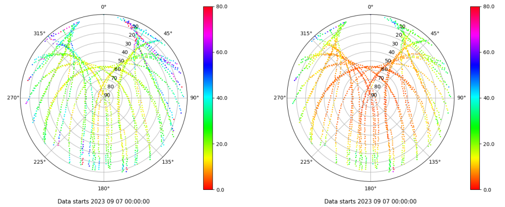
Skyplot for station SPAB. Parameter M1C Data file SPAB00ESP_R_2023250.xtr Skyplot for station SPAB. Parameter M2P Data file SPAB00ESP_R_2023250.xtr
