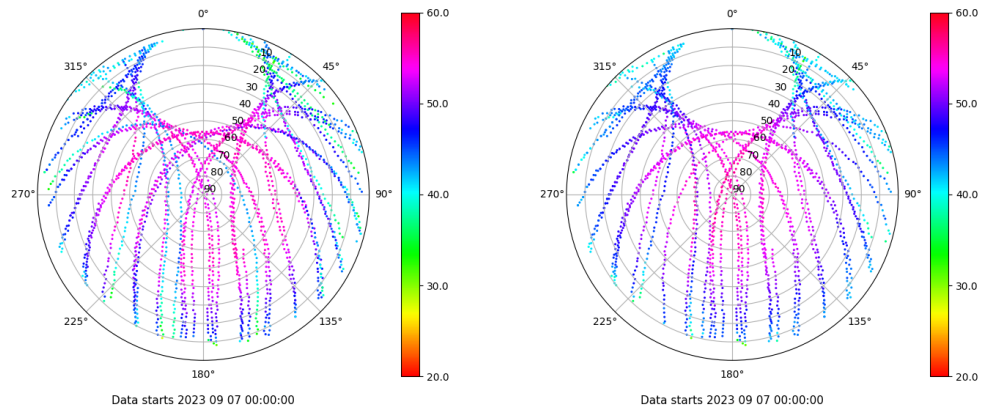
Skyplot for station SPAB. Signal to Noise S1C Data file SPAB00ESP_R_2023250.xtr Skyplot for station SPAB. Signal to Noise S2P Data file SPAB00ESP_R_2023250.xtr
