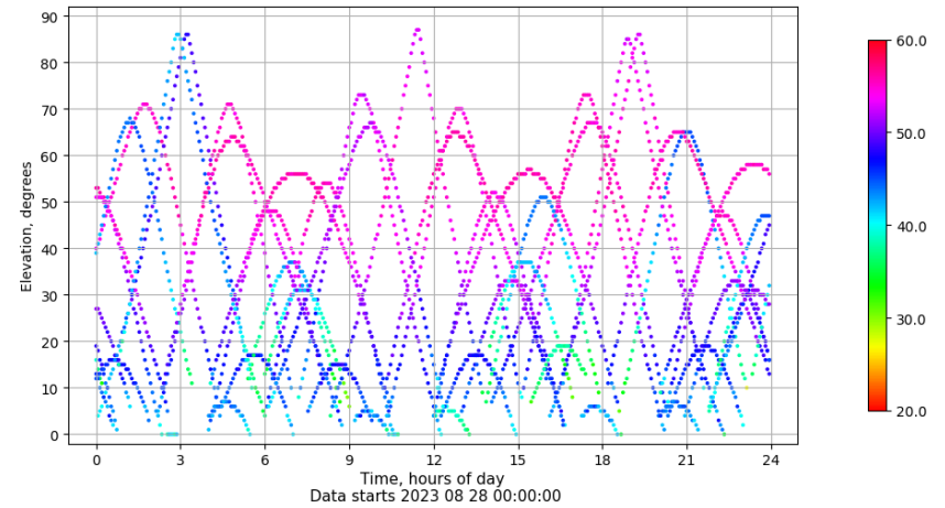
Time-elevation plot for station SPAB. Signal to Noise S1C Data file SPAB00ESP_R_2023240.xtr
