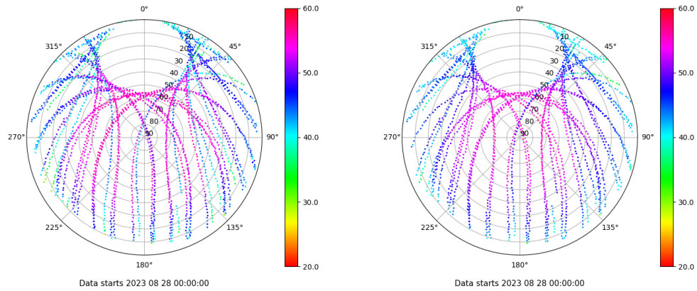
Skyplot for station SPAB. Signal to Noise S1C Data file SPAB00ESP_R_2023240.xtr Skyplot for station SPAB. Signal to Noise S2P Data file SPAB00ESP_R_2023240.xtr
