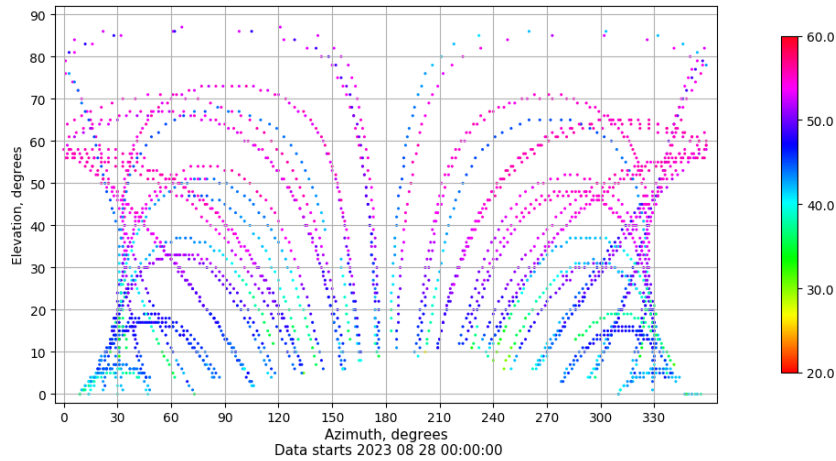
Azimuth-elevation plot for station SPAB. Signal to Noise S1C Data file SPAB00ESP_R_2023240.xtr
