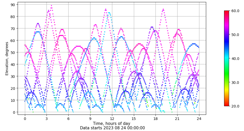
Time-elevation plot for station SPAB. Signal to Noise S1C Data file SPAB00ESP_R_2023236.xtr
