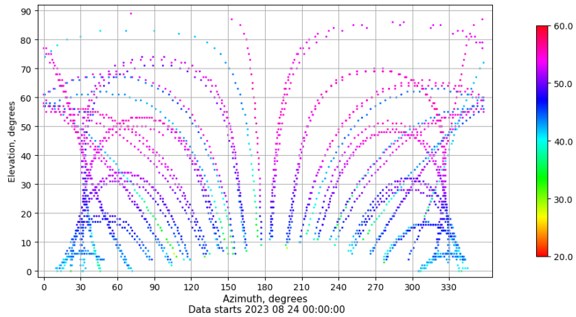
Azimuth-elevation plot for station SPAB. Signal to Noise S1C Data file SPAB00ESP_R_2023236.xtr
