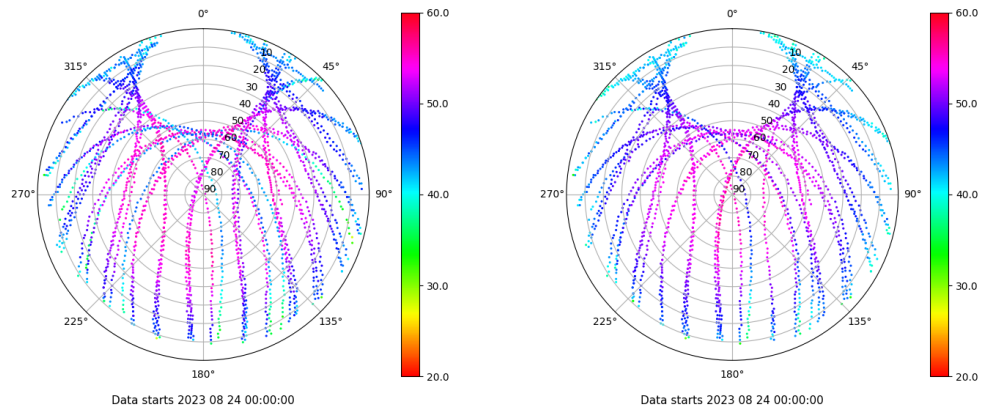
Skyplot for station SPAB. Signal to Noise S1C Data file SPAB00ESP_R_2023236.xtr Skyplot for station SPAB. Signal to Noise S2P Data file SPAB00ESP_R_2023236.xtr
