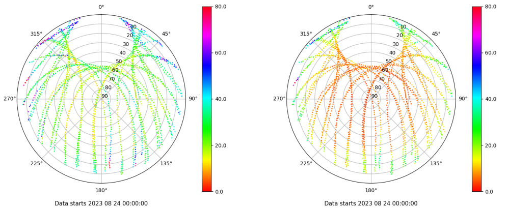
Skyplot for station SPAB. Parameter M1C Data file SPAB00ESP_R_2023236.xtr Skyplot for station SPAB. Parameter M2P Data file SPAB00ESP_R_2023236.xtr
