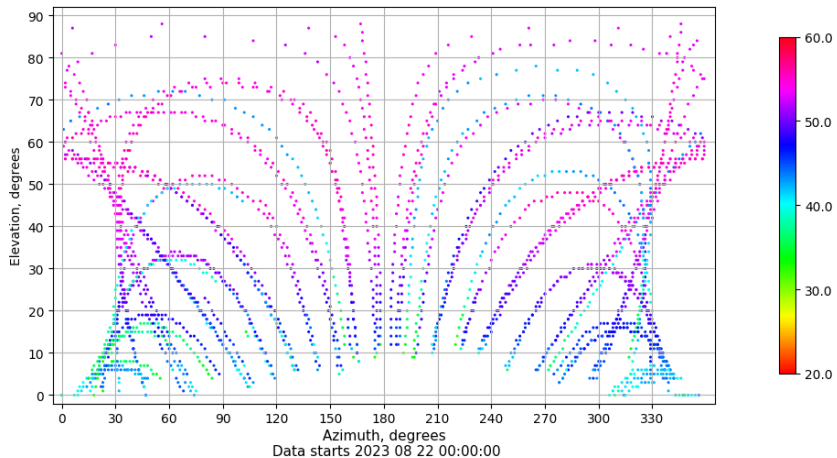
Azimuth-elevation plot for station SPAB. Signal to Noise S1C Data file SPAB00ESP_R_2023234.xtr
