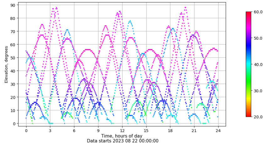
Time-elevation plot for station SPAB. Signal to Noise S1C Data file SPAB00ESP_R_2023234.xtr
