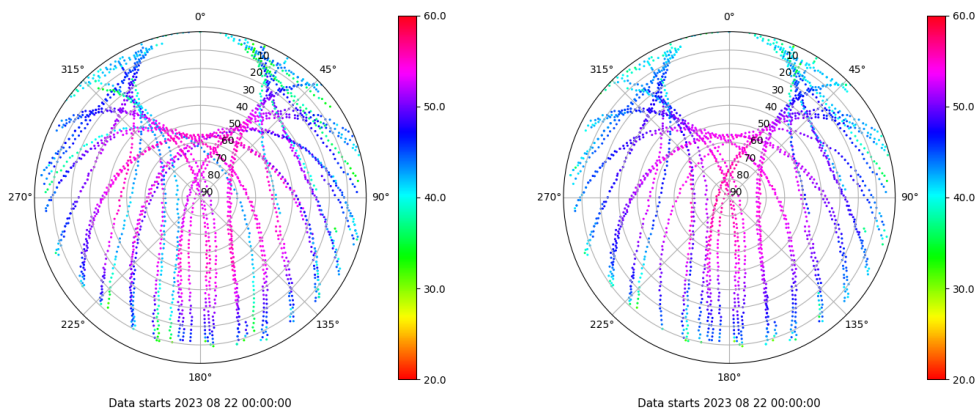
Skyplot for station SPAB. Signal to Noise S1C Data file SPAB00ESP_R_2023234.xtr Skyplot for station SPAB. Signal to Noise S2P Data file SPAB00ESP_R_2023234.xtr
