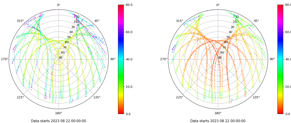
Skyplot for station SPAB. Parameter M1C Data file SPAB00ESP_R_2023234.xtr Skyplot for station SPAB. Parameter M2P Data file SPAB00ESP_R_2023234.xtr
