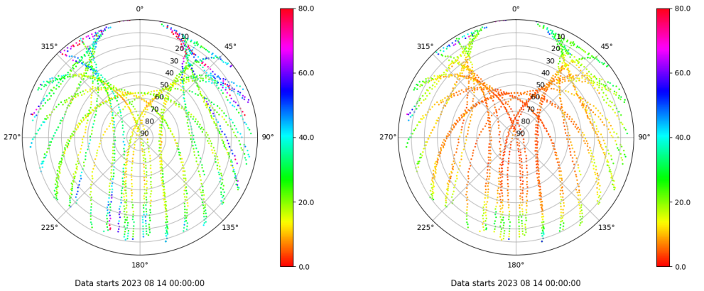
Skyplot for station SPAB. Parameter M1C Data file SPAB00ESP_R_2023226.xtr Skyplot for station SPAB. Parameter M2P Data file SPAB00ESP_R_2023226.xtr
