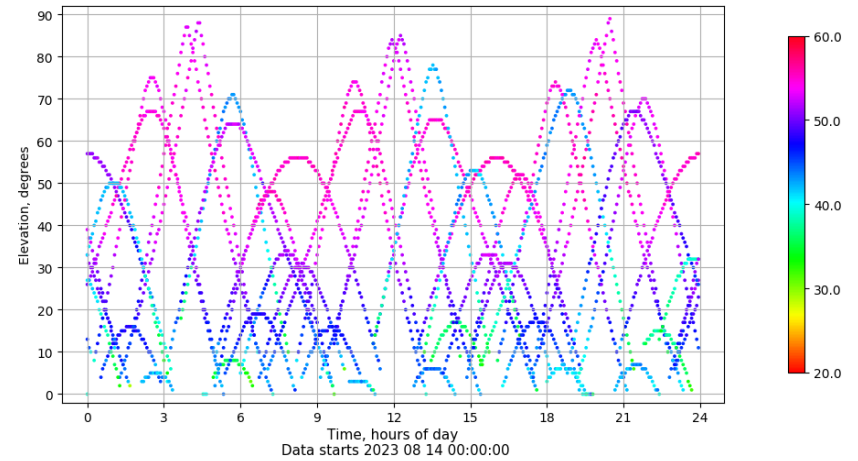
Time-elevation plot for station SPAB. Signal to Noise S1C Data file SPAB00ESP_R_2023226.xtr
