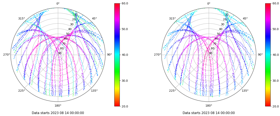
Skyplot for station SPAB. Signal to Noise S1C Data file SPAB00ESP_R_2023226.xtr Skyplot for station SPAB. Signal to Noise S2P Data file SPAB00ESP_R_2023226.xtr
