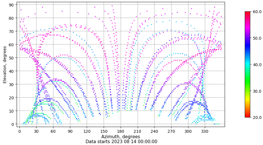
Azimuth-elevation plot for station SPAB. Signal to Noise S1C Data file SPAB00ESP_R_2023226.xtr
