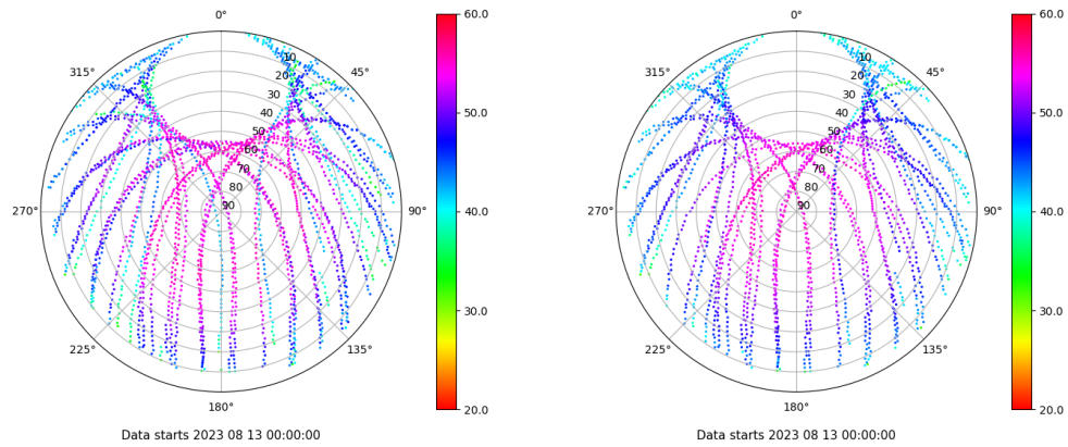
Skyplot for station SPAB. Signal to Noise S1C Data file SPAB00ESP_R_2023225.xtr Skyplot for station SPAB. Signal to Noise S2P Data file SPAB00ESP_R_2023225.xtr
