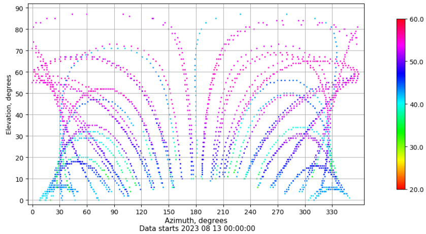
Azimuth-elevation plot for station SPAB. Signal to Noise S1C Data file SPAB00ESP_R_2023225.xtr
