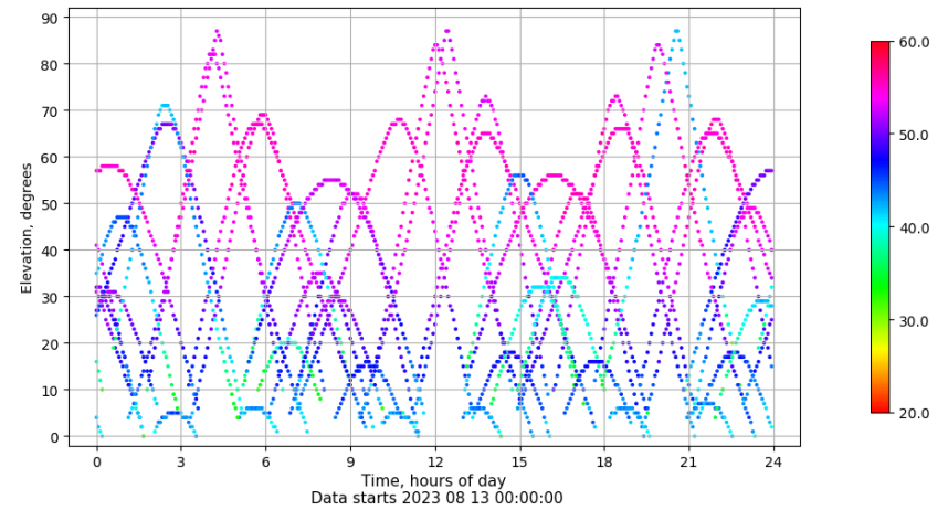
Time-elevation plot for station SPAB. Signal to Noise S1C Data file SPAB00ESP_R_2023225.xtr
