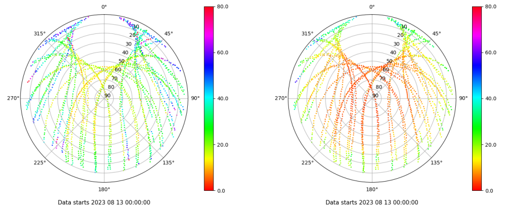
Skyplot for station SPAB. Parameter M1C Data file SPAB00ESP_R_2023225.xtr Skyplot for station SPAB. Parameter M2P Data file SPAB00ESP_R_2023225.xtr
