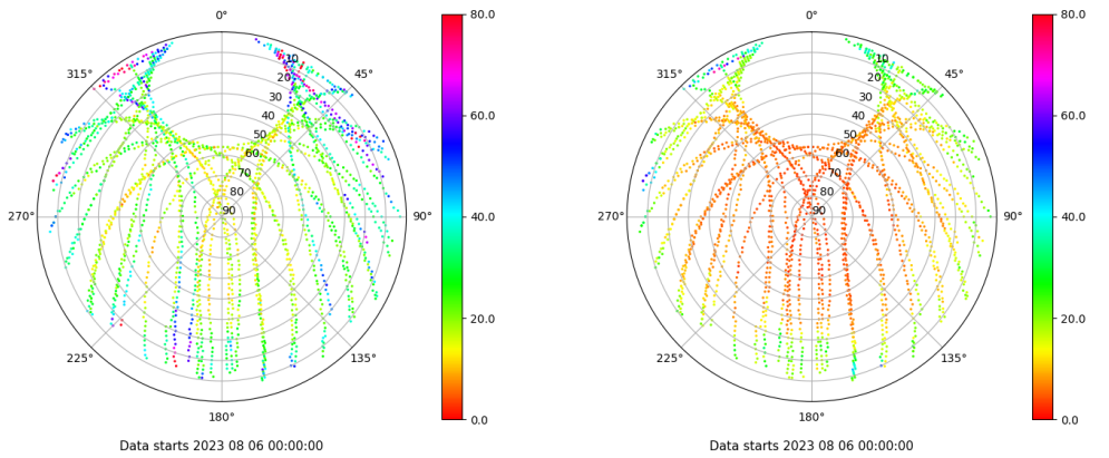
Skyplot for station SPAB. Parameter M1C Data file SPAB00ESP_R_2023218.xtr Skyplot for station SPAB. Parameter M2P Data file SPAB00ESP_R_2023218.xtr
