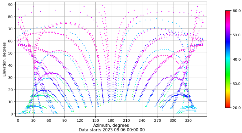
Azimuth-elevation plot for station SPAB. Signal to Noise S1C Data file SPAB00ESP_R_2023218.xtr
