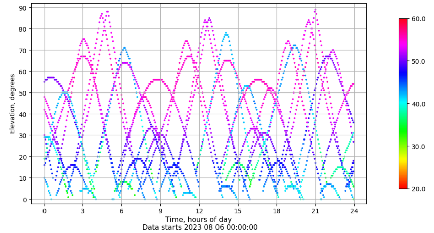
Time-elevation plot for station SPAB. Signal to Noise S1C Data file SPAB00ESP_R_2023218.xtr
