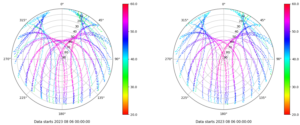
Skyplot for station SPAB. Signal to Noise S1C Data file SPAB00ESP_R_2023218.xtr Skyplot for station SPAB. Signal to Noise S2P Data file SPAB00ESP_R_2023218.xtr
