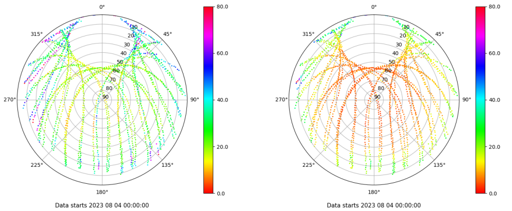
Skyplot for station SPAB. Parameter M1C Data file SPAB00ESP_R_2023216.xtr Skyplot for station SPAB. Parameter M2P Data file SPAB00ESP_R_2023216.xtr
