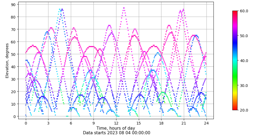
Time-elevation plot for station SPAB. Signal to Noise S1C Data file SPAB00ESP_R_2023216.xtr
