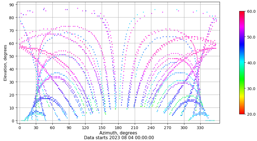
Azimuth-elevation plot for station SPAB. Signal to Noise S1C Data file SPAB00ESP_R_2023216.xtr
