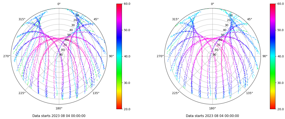
Skyplot for station SPAB. Signal to Noise S1C Data file SPAB00ESP_R_2023216.xtr Skyplot for station SPAB. Signal to Noise S2P Data file SPAB00ESP_R_2023216.xtr
