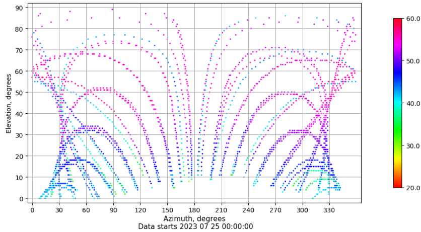
Azimuth-elevation plot for station SPAB. Signal to Noise S1C Data file SPAB00ESP_R_2023206.xtr
