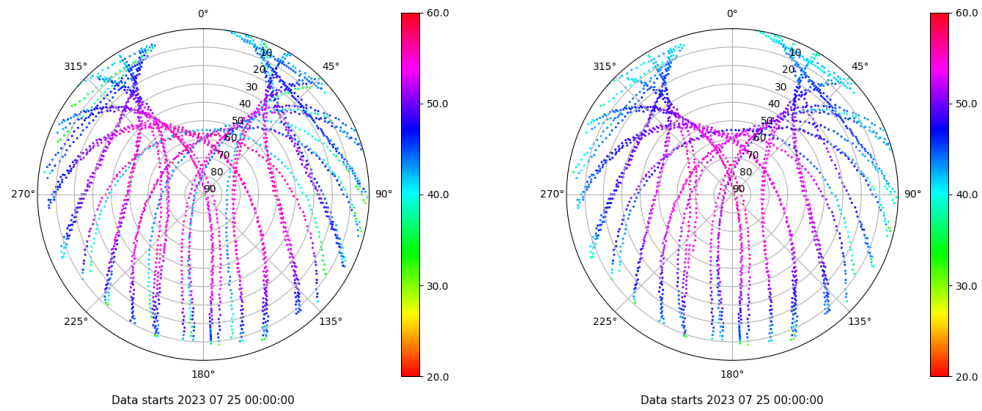
Skyplot for station SPAB. Signal to Noise S1C Data file SPAB00ESP_R_2023206.xtr Skyplot for station SPAB. Signal to Noise S2P Data file SPAB00ESP_R_2023206.xtr
