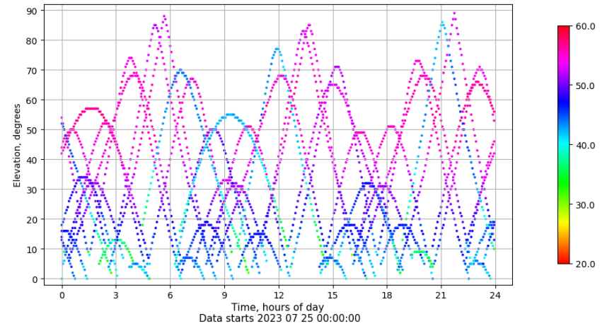
Time-elevation plot for station SPAB. Signal to Noise S1C Data file SPAB00ESP_R_2023206.xtr
