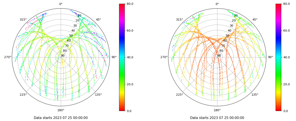
Skyplot for station SPAB. Parameter M1C Data file SPAB00ESP_R_2023206.xtr Skyplot for station SPAB. Parameter M2P Data file SPAB00ESP_R_2023206.xtr
