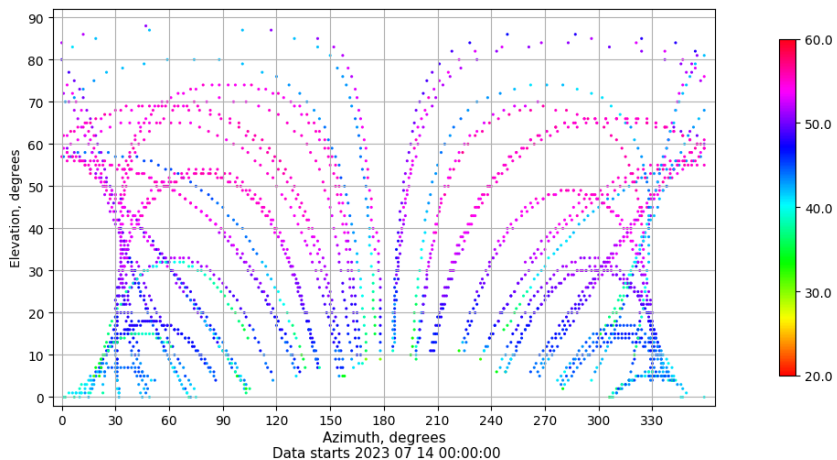
Azimuth-elevation plot for station SPAB. Signal to Noise S1C Data file SPAB00ESP_R_2023195.xtr
