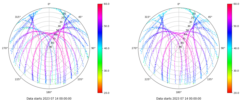
Skyplot for station SPAB. Signal to Noise S1C Data file SPAB00ESP_R_2023195.xtr Skyplot for station SPAB. Signal to Noise S2P Data file SPAB00ESP_R_2023195.xtr
