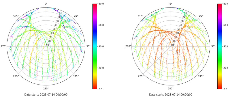
Skyplot for station SPAB. Parameter M1C Data file SPAB00ESP_R_2023195.xtr Skyplot for station SPAB. Parameter M2P Data file SPAB00ESP_R_2023195.xtr
