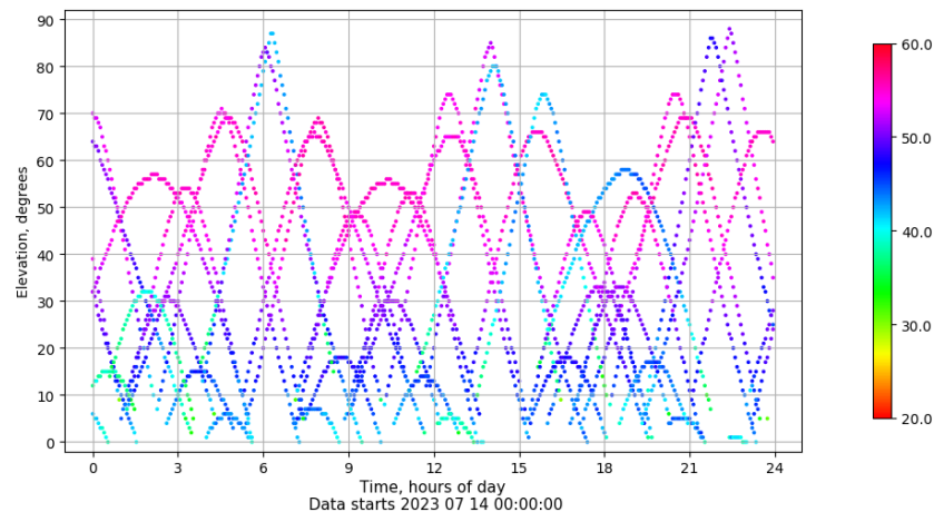
Time-elevation plot for station SPAB. Signal to Noise S1C Data file SPAB00ESP_R_2023195.xtr
