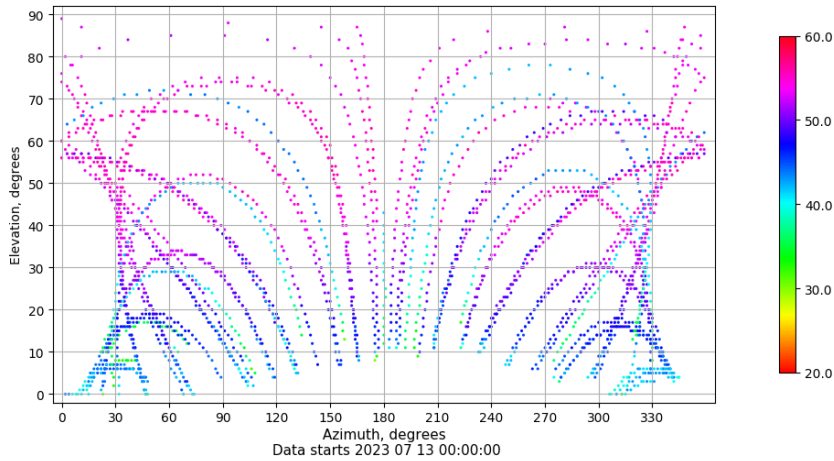
Azimuth-elevation plot for station SPAB. Signal to Noise S1C Data file SPAB00ESP_R_2023194.xtr
