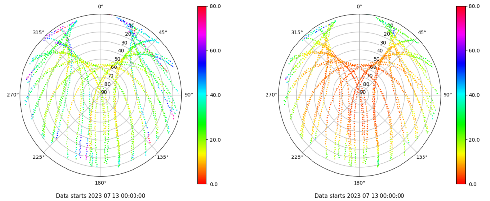
Skyplot for station SPAB. Parameter M1C Data file SPAB00ESP_R_2023194.xtr Skyplot for station SPAB. Parameter M2P Data file SPAB00ESP_R_2023194.xtr
