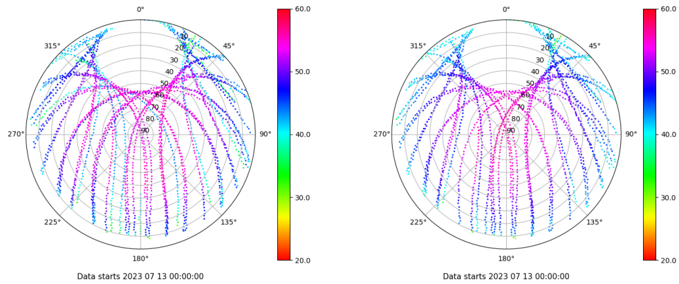
Skyplot for station SPAB. Signal to Noise S1C Data file SPAB00ESP_R_2023194.xtr Skyplot for station SPAB. Signal to Noise S2P Data file SPAB00ESP_R_2023194.xtr
