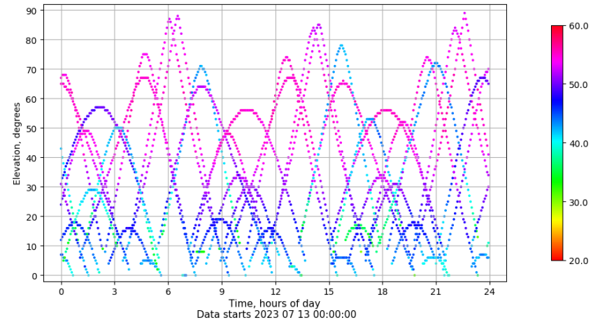
Time-elevation plot for station SPAB. Signal to Noise S1C Data file SPAB00ESP_R_2023194.xtr
