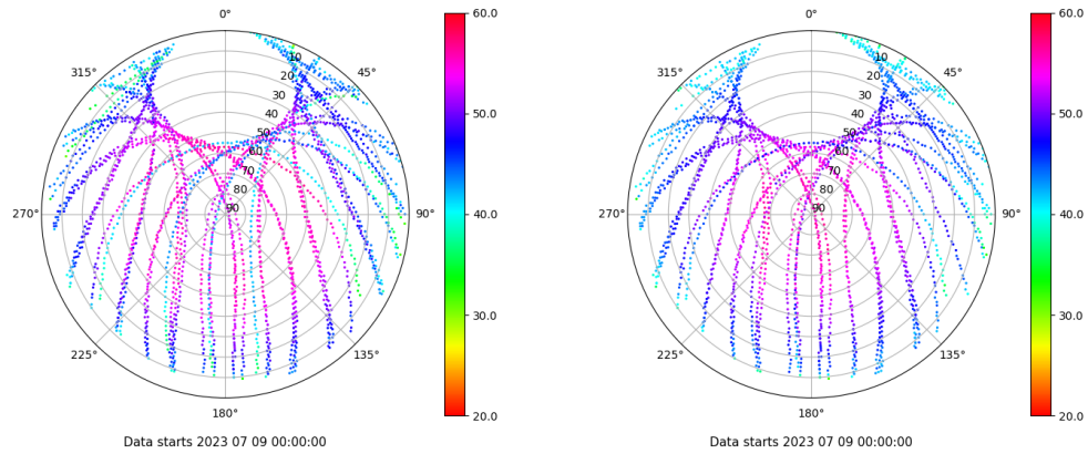
Skyplot for station SPAB. Signal to Noise S1C Data file SPAB00ESP_R_2023190.xtr Skyplot for station SPAB. Signal to Noise S2P Data file SPAB00ESP_R_2023190.xtr
