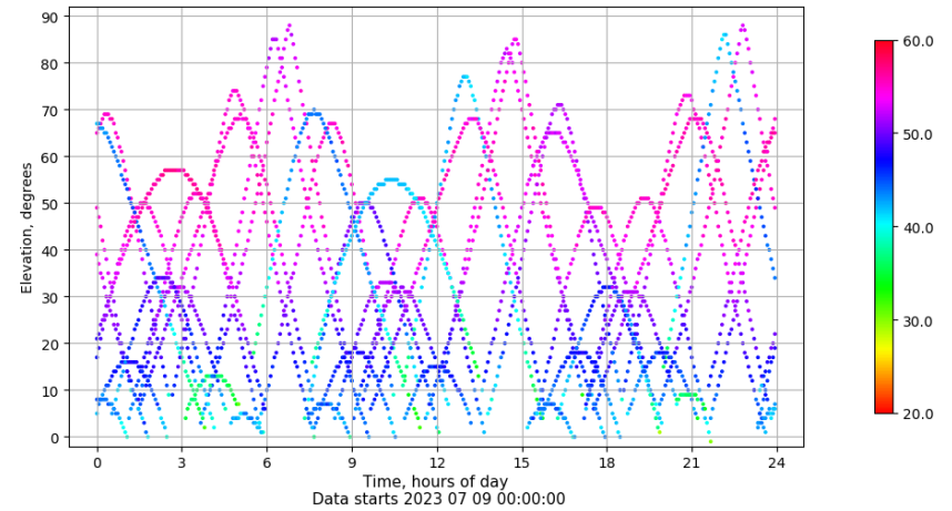
Time-elevation plot for station SPAB. Signal to Noise S1C Data file SPAB00ESP_R_2023190.xtr
