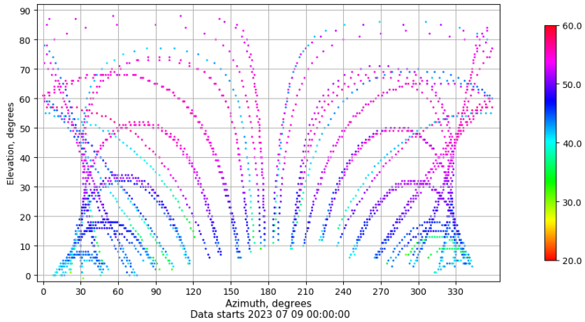
Azimuth-elevation plot for station SPAB. Signal to Noise S1C Data file SPAB00ESP_R_2023190.xtr
