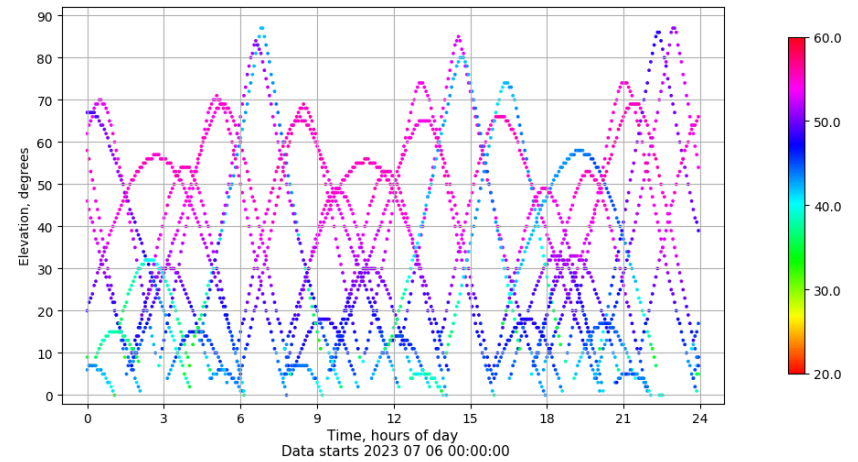
Time-elevation plot for station SPAB. Signal to Noise S1C Data file SPAB00ESP_R_2023187.xtr
