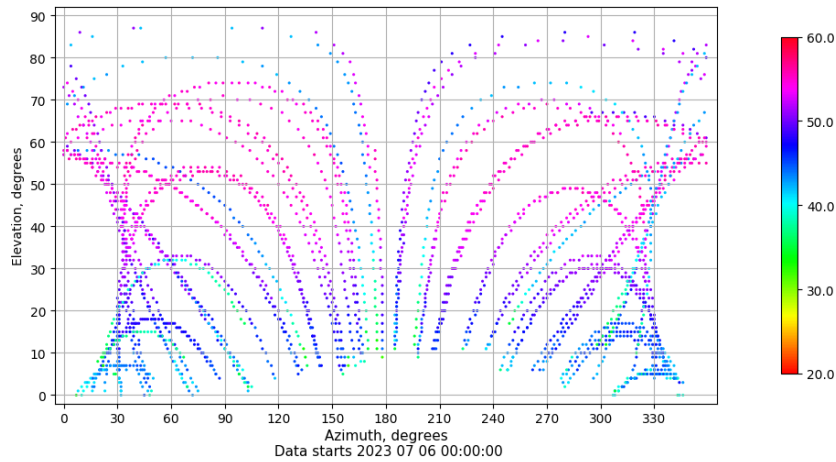
Azimuth-elevation plot for station SPAB. Signal to Noise S1C Data file SPAB00ESP_R_2023187.xtr
