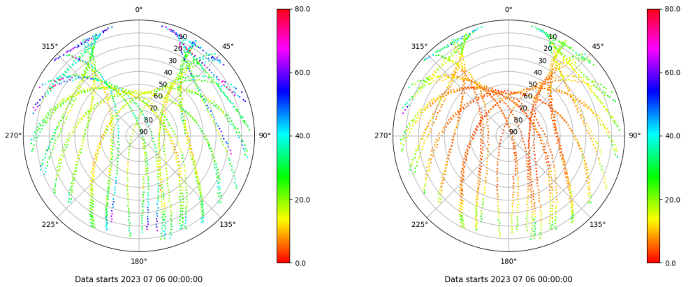
Skyplot for station SPAB. Parameter M1C Data file SPAB00ESP_R_2023187.xtr Skyplot for station SPAB. Parameter M2P Data file SPAB00ESP_R_2023187.xtr
