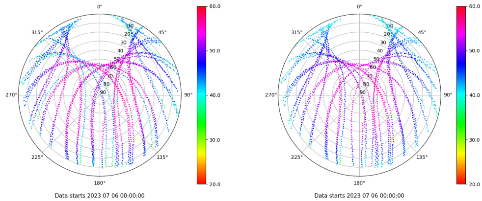
Skyplot for station SPAB. Signal to Noise S1C Data file SPAB00ESP_R_2023187.xtr Skyplot for station SPAB. Signal to Noise S2P Data file SPAB00ESP_R_2023187.xtr
