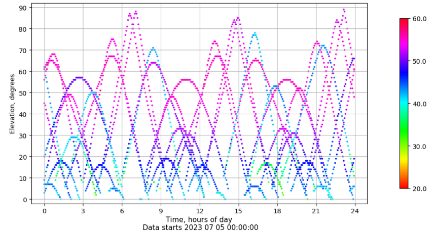
Time-elevation plot for station SPAB. Signal to Noise S1C Data file SPAB00ESP_R_2023186.xtr
