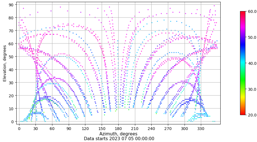
Azimuth-elevation plot for station SPAB. Signal to Noise S1C Data file SPAB00ESP_R_2023186.xtr
