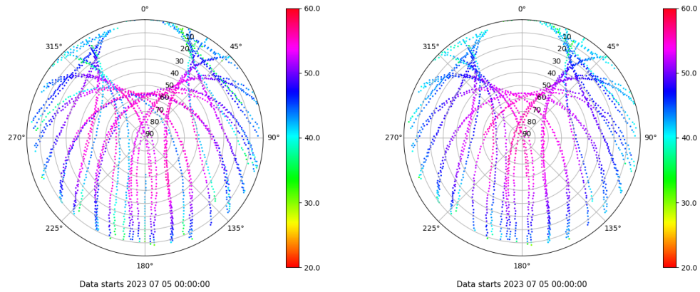
Skyplot for station SPAB. Signal to Noise S1C Data file SPAB00ESP_R_2023186.xtr Skyplot for station SPAB. Signal to Noise S2P Data file SPAB00ESP_R_2023186.xtr
