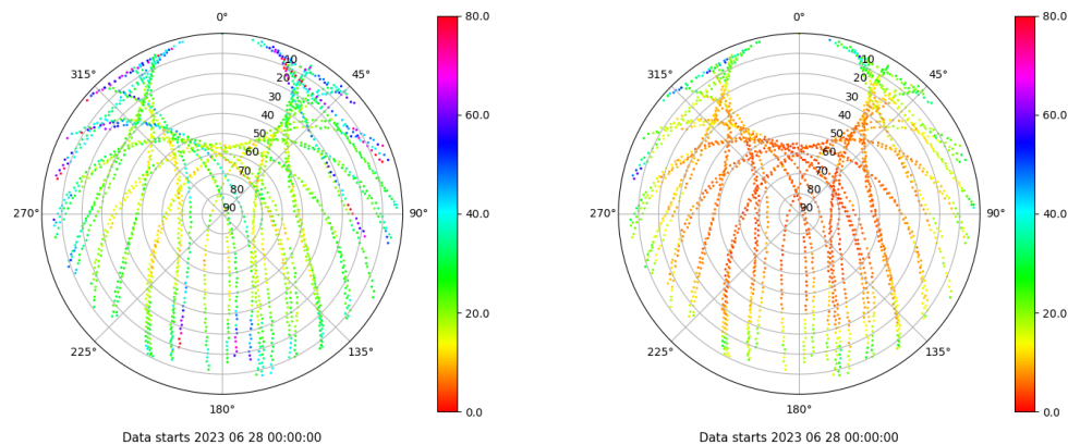
Skyplot for station SPAB. Parameter M1C Data file SPAB00ESP_R_2023179.xtr Skyplot for station SPAB. Parameter M2P Data file SPAB00ESP_R_2023179.xtr
