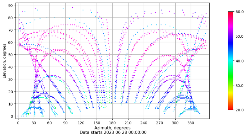
Azimuth-elevation plot for station SPAB. Signal to Noise S1C Data file SPAB00ESP_R_2023179.xtr
