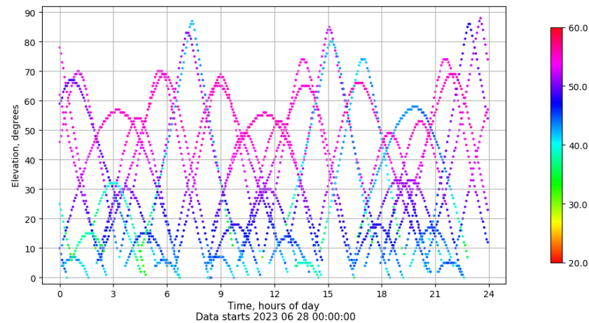
Time-elevation plot for station SPAB. Signal to Noise S1C Data file SPAB00ESP_R_2023179.xtr
