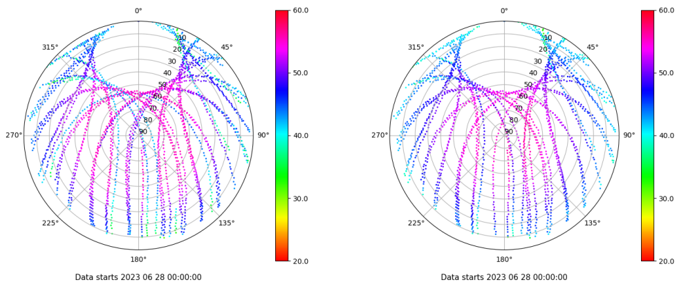
Skyplot for station SPAB. Signal to Noise S1C Data file SPAB00ESP_R_2023179.xtr Skyplot for station SPAB. Signal to Noise S2P Data file SPAB00ESP_R_2023179.xtr
