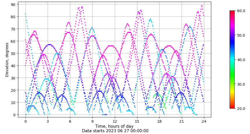
Time-elevation plot for station SPAB. Signal to Noise S1C Data file SPAB00ESP_R_2023178.xtr
