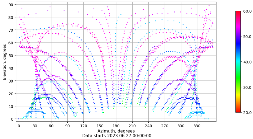
Azimuth-elevation plot for station SPAB. Signal to Noise S1C Data file SPAB00ESP_R_2023178.xtr
