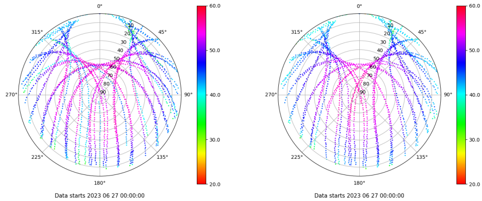
Skyplot for station SPAB. Signal to Noise S1C Data file SPAB00ESP_R_2023178.xtr Skyplot for station SPAB. Signal to Noise S2P Data file SPAB00ESP_R_2023178.xtr
