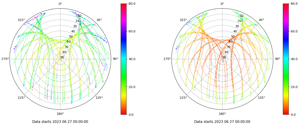
Skyplot for station SPAB. Parameter M1C Data file SPAB00ESP_R_2023178.xtr Skyplot for station SPAB. Parameter M2P Data file SPAB00ESP_R_2023178.xtr
