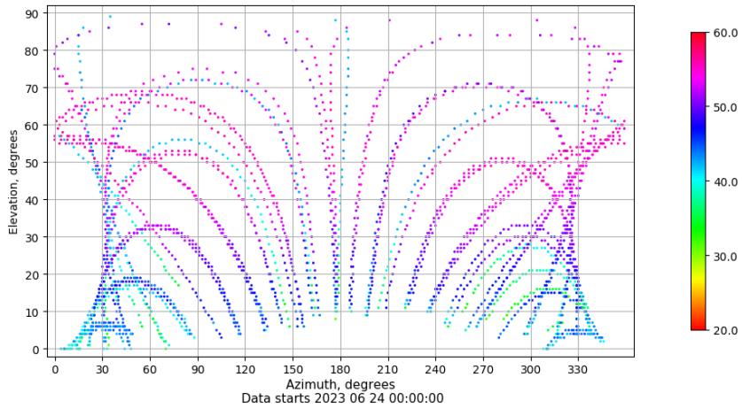
Azimuth-elevation plot for station SPAB. Signal to Noise S1C Data file SPAB00ESP_R_2023175.xtr
