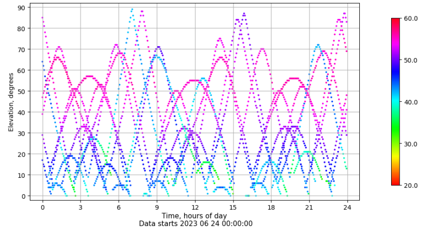
Time-elevation plot for station SPAB. Signal to Noise S1C Data file SPAB00ESP_R_2023175.xtr
