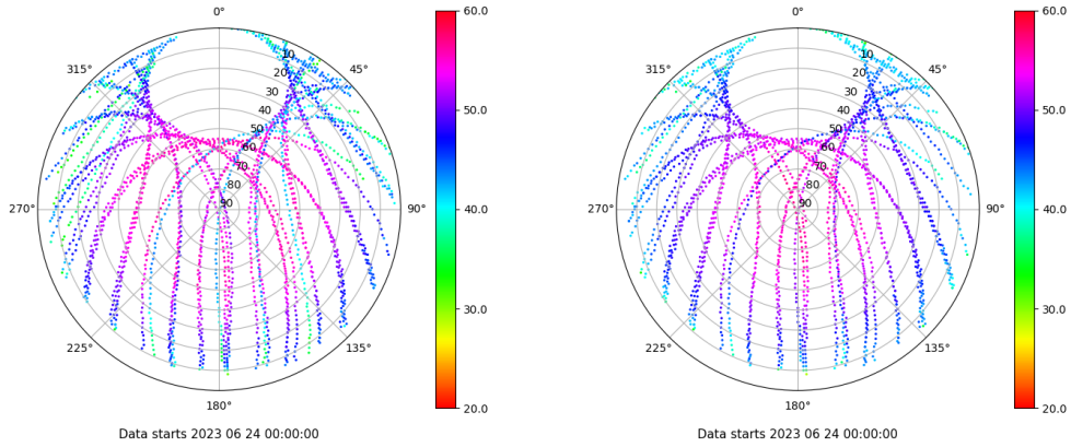
Skyplot for station SPAB. Signal to Noise S1C Data file SPAB00ESP_R_2023175.xtr Skyplot for station SPAB. Signal to Noise S2P Data file SPAB00ESP_R_2023175.xtr
