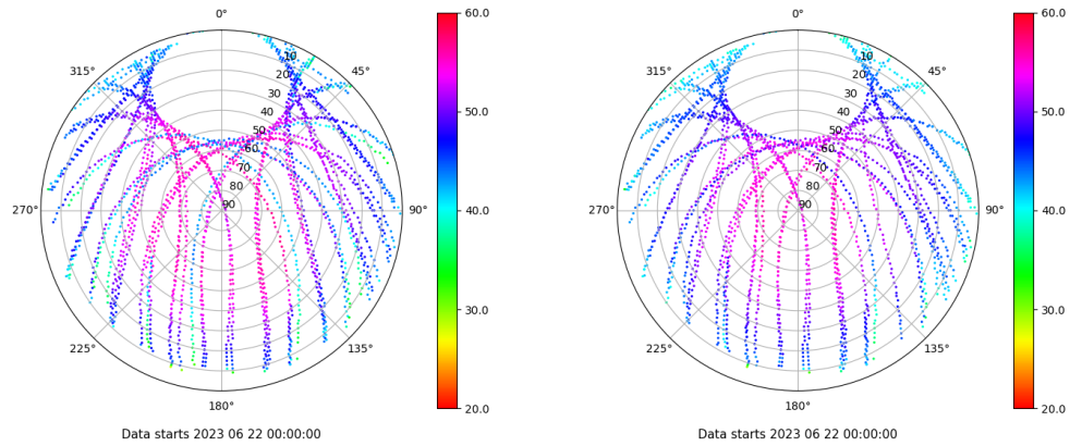
Skyplot for station SPAB. Signal to Noise S1C Data file SPAB00ESP_R_2023173.xtr Skyplot for station SPAB. Signal to Noise S2P Data file SPAB00ESP_R_2023173.xtr
