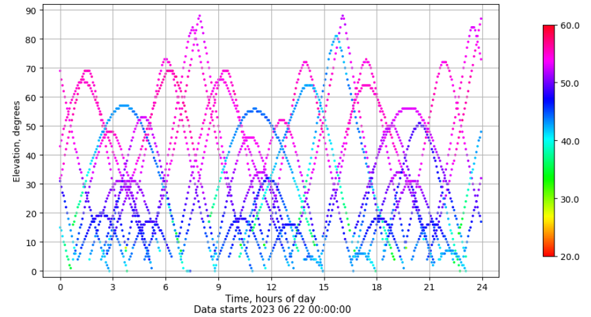
Time-elevation plot for station SPAB. Signal to Noise S1C Data file SPAB00ESP_R_2023173.xtr
