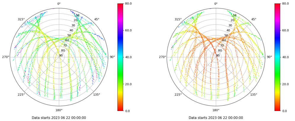
Skyplot for station SPAB. Parameter M1C Data file SPAB00ESP_R_2023173.xtr Skyplot for station SPAB. Parameter M2P Data file SPAB00ESP_R_2023173.xtr
