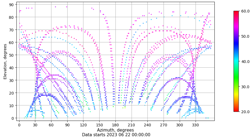
Azimuth-elevation plot for station SPAB. Signal to Noise S1C Data file SPAB00ESP_R_2023173.xtr
