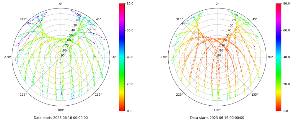
Skyplot for station SPAB. Parameter M1C Data file SPAB00ESP_R_2023167.xtr Skyplot for station SPAB. Parameter M2P Data file SPAB00ESP_R_2023167.xtr
