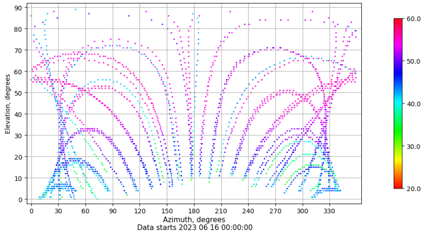
Azimuth-elevation plot for station SPAB. Signal to Noise S1C Data file SPAB00ESP_R_2023167.xtr
