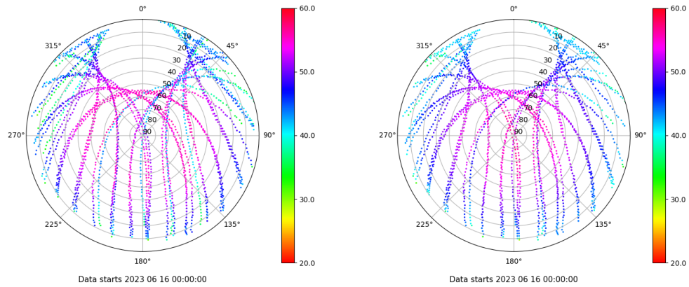
Skyplot for station SPAB. Signal to Noise S1C Data file SPAB00ESP_R_2023167.xtr Skyplot for station SPAB. Signal to Noise S2P Data file SPAB00ESP_R_2023167.xtr
