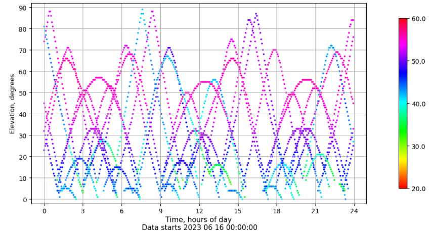
Time-elevation plot for station SPAB. Signal to Noise S1C Data file SPAB00ESP_R_2023167.xtr
