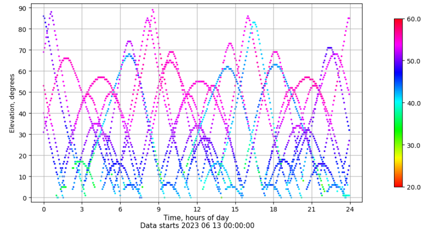
Time-elevation plot for station SPAB. Signal to Noise S1C Data file SPAB00ESP_R_2023164.xtr
