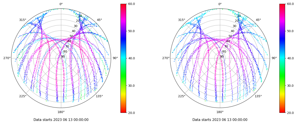
Skyplot for station SPAB. Signal to Noise S1C Data file SPAB00ESP_R_2023164.xtr Skyplot for station SPAB. Signal to Noise S2P Data file SPAB00ESP_R_2023164.xtr
