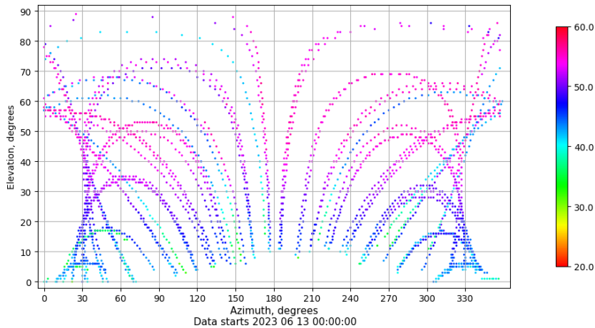
Azimuth-elevation plot for station SPAB. Signal to Noise S1C Data file SPAB00ESP_R_2023164.xtr
