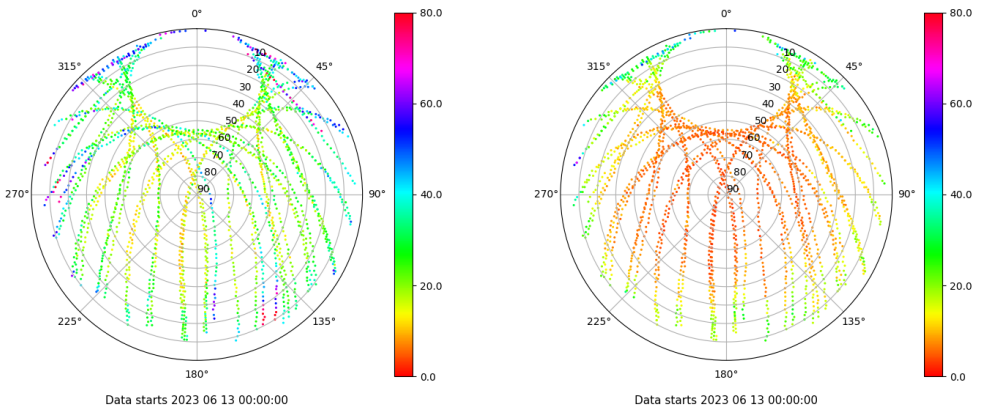
Skyplot for station SPAB. Parameter M1C Data file SPAB00ESP_R_2023164.xtr Skyplot for station SPAB. Parameter M2P Data file SPAB00ESP_R_2023164.xtr
