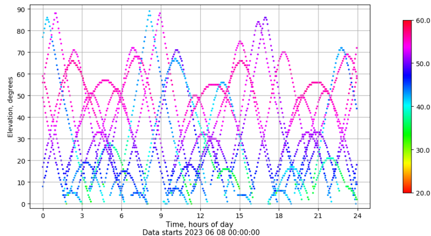
Time-elevation plot for station SPAB. Signal to Noise S1C Data file SPAB00ESP_R_2023159.xtr
