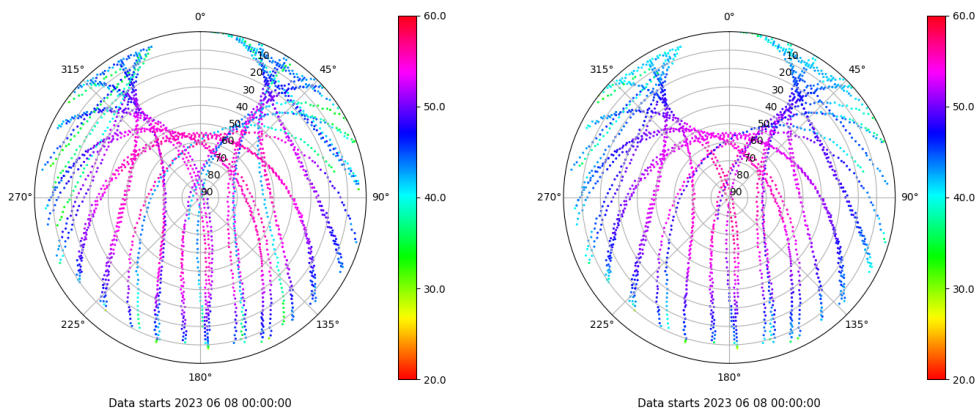
Skyplot for station SPAB. Signal to Noise S1C Data file SPAB00ESP_R_2023159.xtr Skyplot for station SPAB. Signal to Noise S2P Data file SPAB00ESP_R_2023159.xtr
