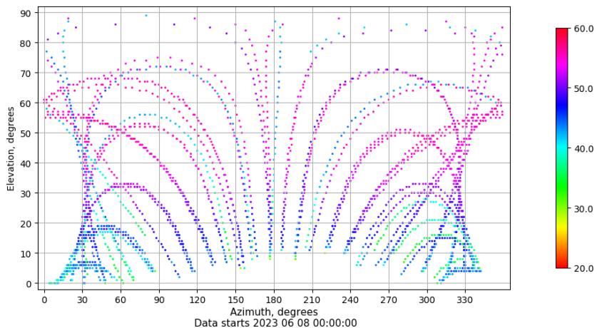
Azimuth-elevation plot for station SPAB. Signal to Noise S1C Data file SPAB00ESP_R_2023159.xtr
