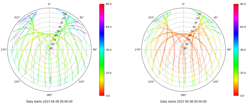
Skyplot for station SPAB. Parameter M1C Data file SPAB00ESP_R_2023159.xtr Skyplot for station SPAB. Parameter M2P Data file SPAB00ESP_R_2023159.xtr
