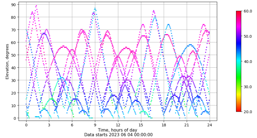
Time-elevation plot for station SPAB. Signal to Noise S1C Data file SPAB00ESP_R_2023155.xtr
