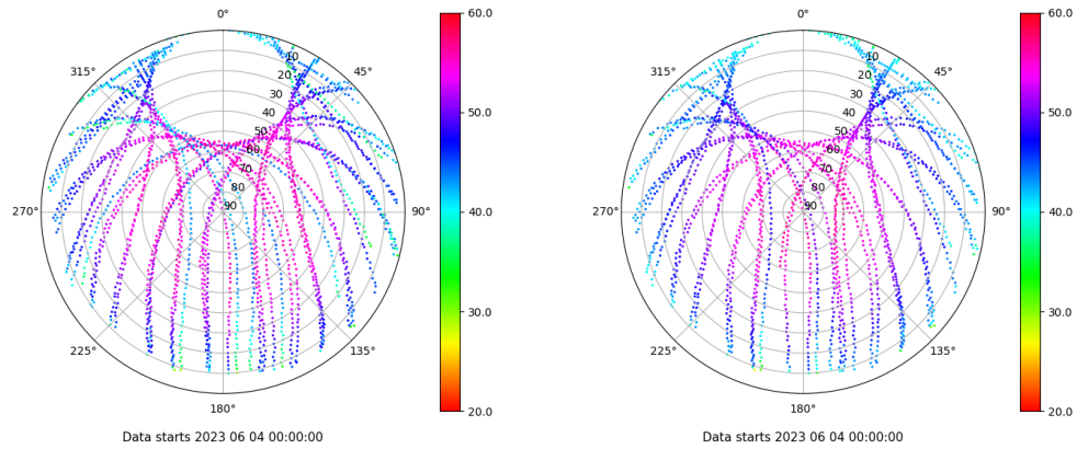
Skyplot for station SPAB. Signal to Noise S1C Data file SPAB00ESP_R_2023155.xtr Skyplot for station SPAB. Signal to Noise S2P Data file SPAB00ESP_R_2023155.xtr
