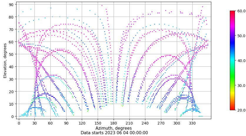
Azimuth-elevation plot for station SPAB. Signal to Noise S1C Data file SPAB00ESP_R_2023155.xtr
