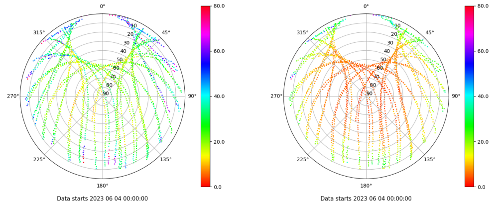
Skyplot for station SPAB. Parameter M1C Data file SPAB00ESP_R_2023155.xtr Skyplot for station SPAB. Parameter M2P Data file SPAB00ESP_R_2023155.xtr
