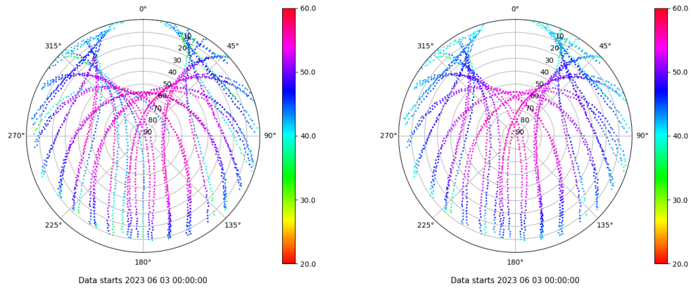
Skyplot for station SPAB. Signal to Noise S1C Data file SPAB00ESP_R_2023154.xtr Skyplot for station SPAB. Signal to Noise S2P Data file SPAB00ESP_R_2023154.xtr
