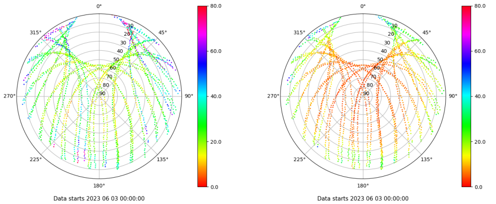
Skyplot for station SPAB. Parameter M1C Data file SPAB00ESP_R_2023154.xtr Skyplot for station SPAB. Parameter M2P Data file SPAB00ESP_R_2023154.xtr
