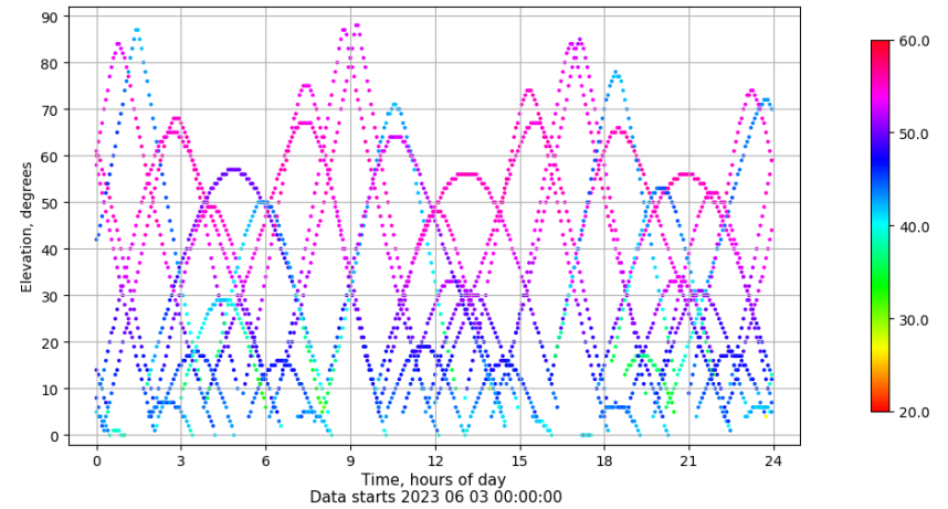
Time-elevation plot for station SPAB. Signal to Noise S1C Data file SPAB00ESP_R_2023154.xtr
