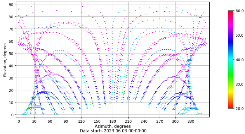
Azimuth-elevation plot for station SPAB. Signal to Noise S1C Data file SPAB00ESP_R_2023154.xtr
