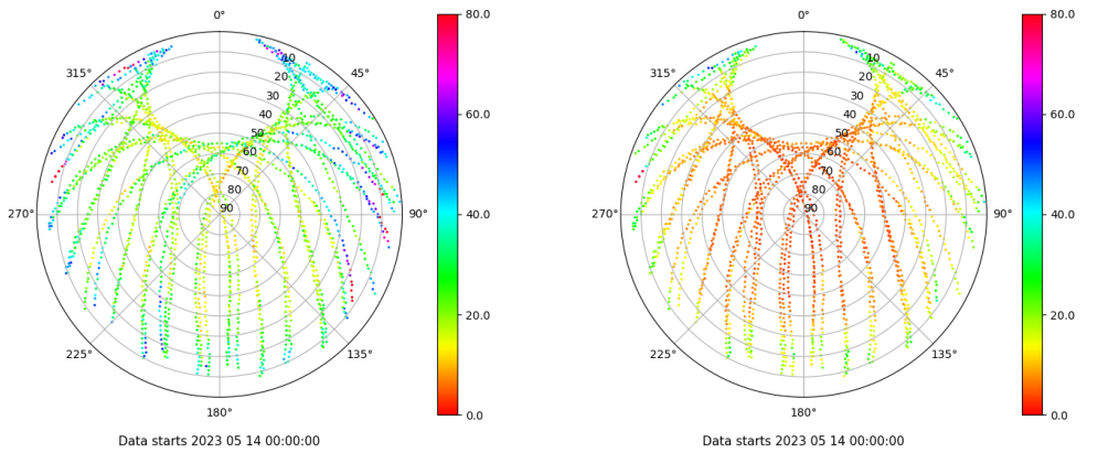
Skyplot for station SPAB. Parameter M1C Data file SPAB00ESP_R_2023134.xtr Skyplot for station SPAB. Parameter M2P Data file SPAB00ESP_R_2023134.xtr
