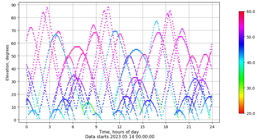
Time-elevation plot for station SPAB. Signal to Noise S1C Data file SPAB00ESP_R_2023134.xtr
