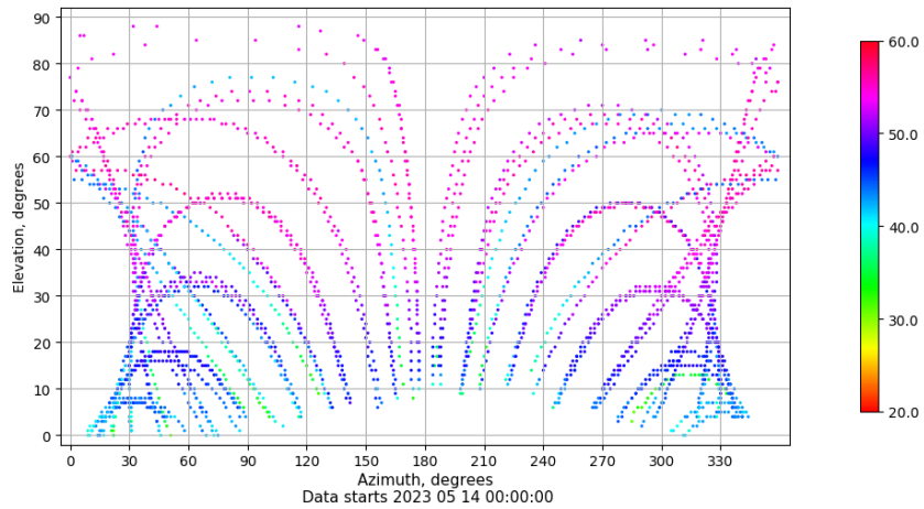
Azimuth-elevation plot for station SPAB. Signal to Noise S1C Data file SPAB00ESP_R_2023134.xtr
