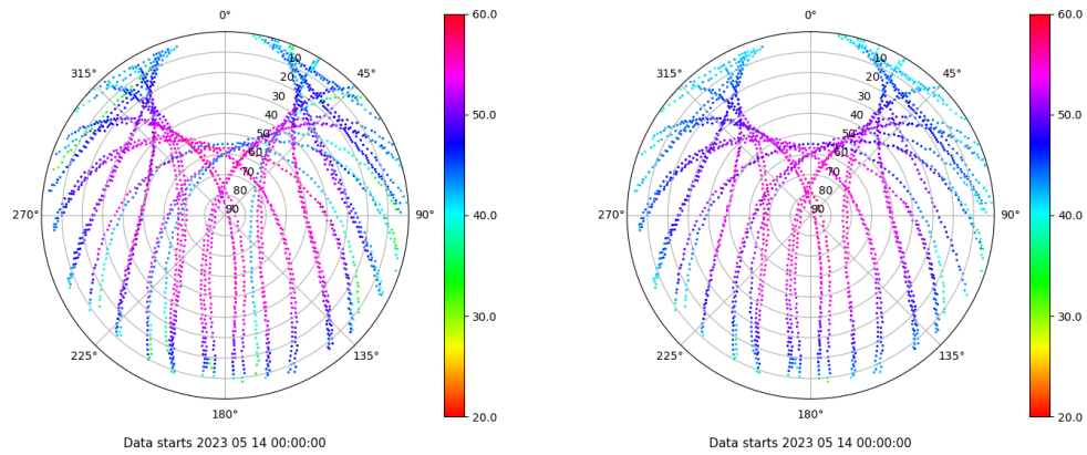
Skyplot for station SPAB. Signal to Noise S1C Data file SPAB00ESP_R_2023134.xtr Skyplot for station SPAB. Signal to Noise S2P Data file SPAB00ESP_R_2023134.xtr
