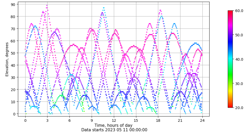
Time-elevation plot for station SPAB. Signal to Noise S1C Data file SPAB00ESP_R_2023131.xtr
