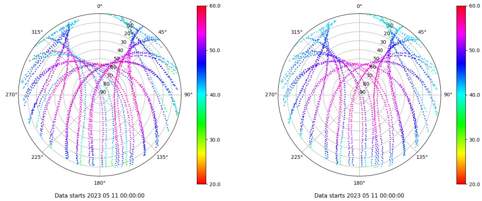
Skyplot for station SPAB. Signal to Noise S1C Data file SPAB00ESP_R_2023131.xtr Skyplot for station SPAB. Signal to Noise S2P Data file SPAB00ESP_R_2023131.xtr
