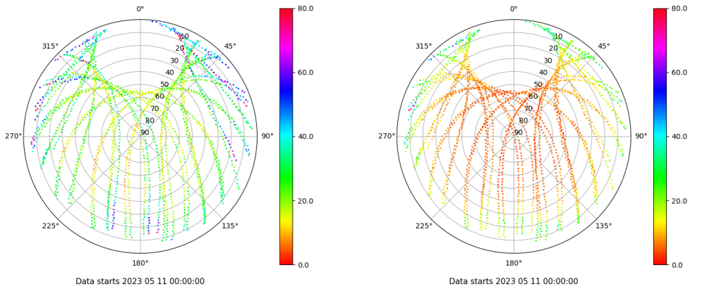
Skyplot for station SPAB. Parameter M1C Data file SPAB00ESP_R_2023131.xtr Skyplot for station SPAB. Parameter M2P Data file SPAB00ESP_R_2023131.xtr
