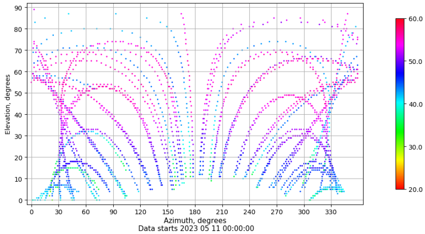
Azimuth-elevation plot for station SPAB. Signal to Noise S1C Data file SPAB00ESP_R_2023131.xtr
