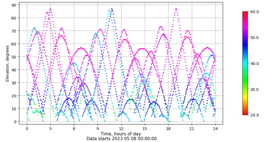
Time-elevation plot for station SPAB. Signal to Noise S1C Data file SPAB00ESP_R_2023128.xtr
