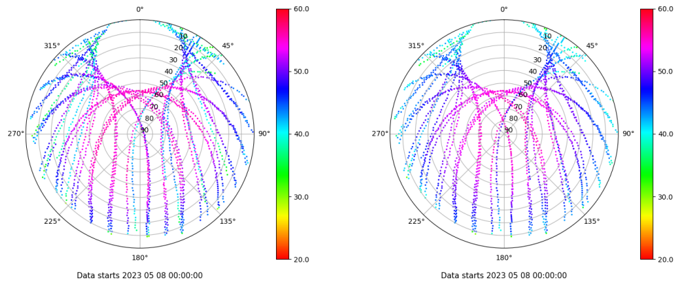
Skyplot for station SPAB. Signal to Noise S1C Data file SPAB00ESP_R_2023128.xtr Skyplot for station SPAB. Signal to Noise S2P Data file SPAB00ESP_R_2023128.xtr
