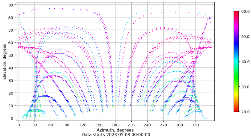
Azimuth-elevation plot for station SPAB. Signal to Noise S1C Data file SPAB00ESP_R_2023128.xtr
