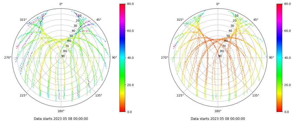
Skyplot for station SPAB. Parameter M1C Data file SPAB00ESP_R_2023128.xtr Skyplot for station SPAB. Parameter M2P Data file SPAB00ESP_R_2023128.xtr
