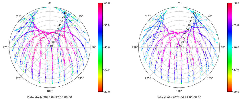
Skyplot for station SPAB. Signal to Noise S1C Data file SPAB00ESP_R_2023112.xtr Skyplot for station SPAB. Signal to Noise S2P Data file SPAB00ESP_R_2023112.xtr
