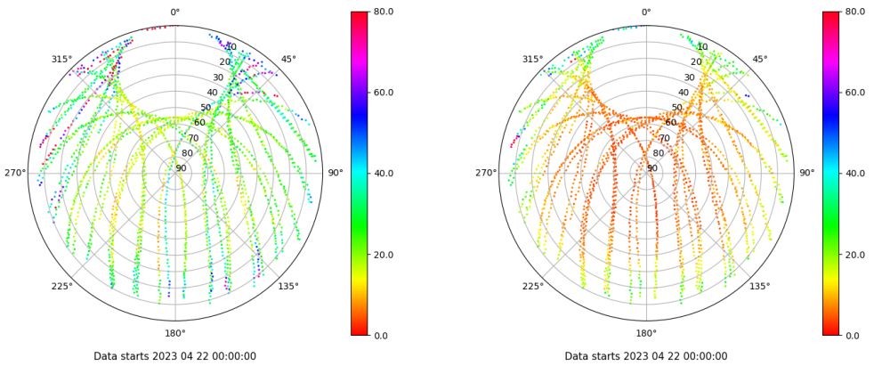
Skyplot for station SPAB. Parameter M1C Data file SPAB00ESP_R_2023112.xtr Skyplot for station SPAB. Parameter M2P Data file SPAB00ESP_R_2023112.xtr
