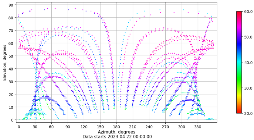
Azimuth-elevation plot for station SPAB. Signal to Noise S1C Data file SPAB00ESP_R_2023112.xtr
