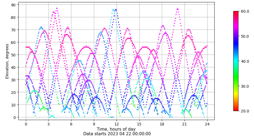
Time-elevation plot for station SPAB. Signal to Noise S1C Data file SPAB00ESP_R_2023112.xtr
