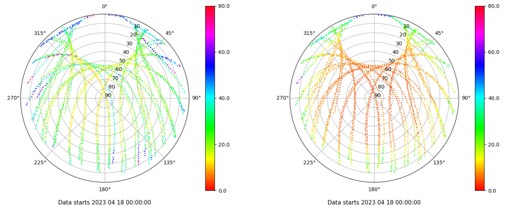
Skyplot for station SPAB. Parameter M1C Data file SPAB00ESP_R_2023108.xtr Skyplot for station SPAB. Parameter M2P Data file SPAB00ESP_R_2023108.xtr
