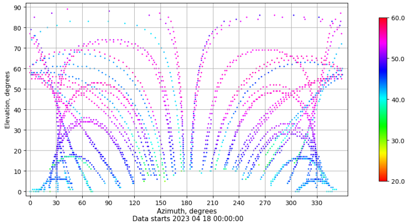
Azimuth-elevation plot for station SPAB. Signal to Noise S1C Data file SPAB00ESP_R_2023108.xtr
