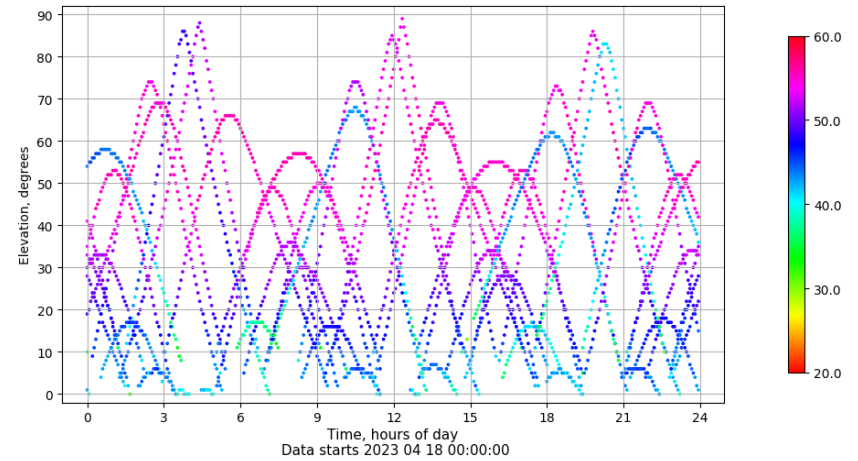
Time-elevation plot for station SPAB. Signal to Noise S1C Data file SPAB00ESP_R_2023108.xtr
