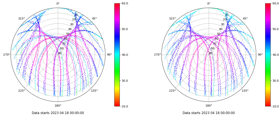
Skyplot for station SPAB. Signal to Noise S1C Data file SPAB00ESP_R_2023108.xtr Skyplot for station SPAB. Signal to Noise S2P Data file SPAB00ESP_R_2023108.xtr
