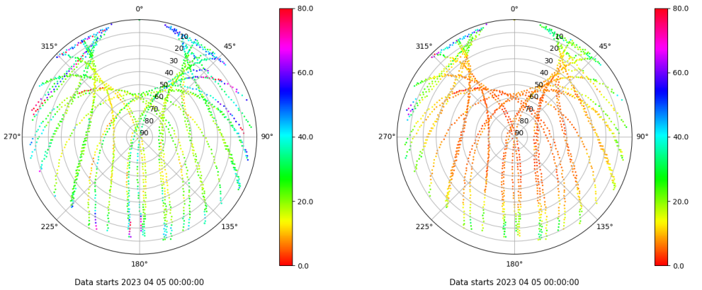
Skyplot for station SPAB. Parameter M1C Data file SPAB00ESP_R_2023095.xtr Skyplot for station SPAB. Parameter M2P Data file SPAB00ESP_R_2023095.xtr
