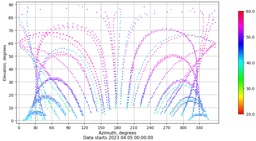
Azimuth-elevation plot for station SPAB. Signal to Noise S1C Data file SPAB00ESP_R_2023095.xtr
