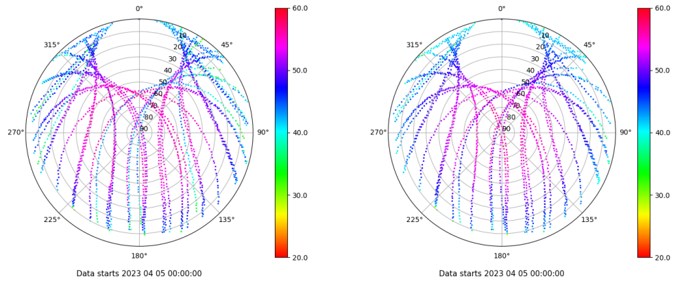
Skyplot for station SPAB. Signal to Noise S1C Data file SPAB00ESP_R_2023095.xtr Skyplot for station SPAB. Signal to Noise S2P Data file SPAB00ESP_R_2023095.xtr
