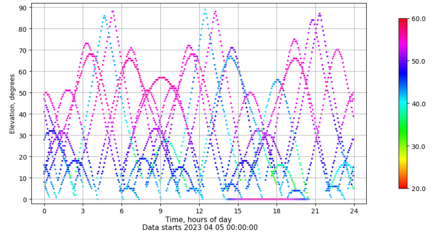
Time-elevation plot for station SPAB. Signal to Noise S1C Data file SPAB00ESP_R_2023095.xtr
