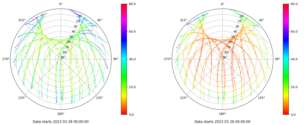
Skyplot for station SPAB. Parameter M1C Data file SPAB00ESP_R_2023087.xtr Skyplot for station SPAB. Parameter M2P Data file SPAB00ESP_R_2023087.xtr
