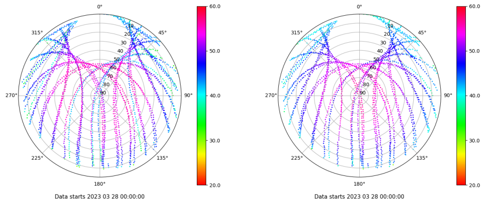
Skyplot for station SPAB. Signal to Noise S1C Data file SPAB00ESP_R_2023087.xtr Skyplot for station SPAB. Signal to Noise S2P Data file SPAB00ESP_R_2023087.xtr
