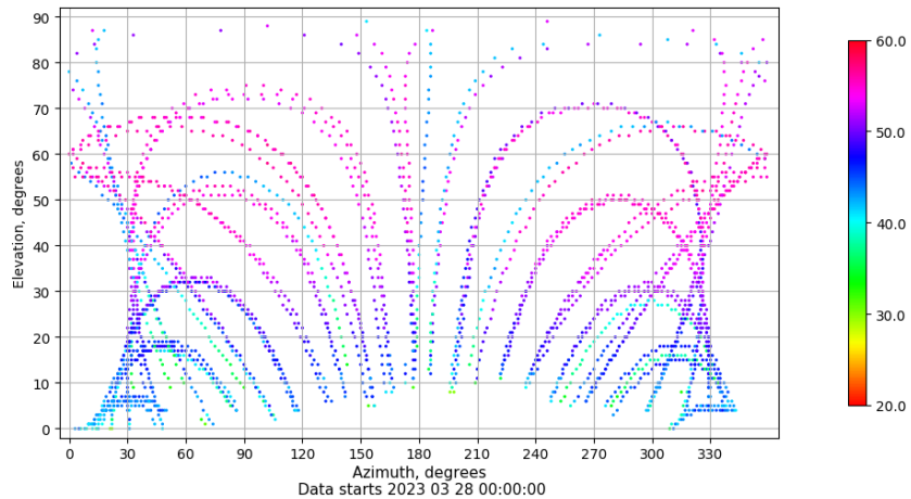
Azimuth-elevation plot for station SPAB. Signal to Noise S1C Data file SPAB00ESP_R_2023087.xtr
