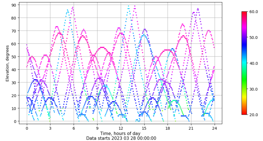
Time-elevation plot for station SPAB. Signal to Noise S1C Data file SPAB00ESP_R_2023087.xtr
