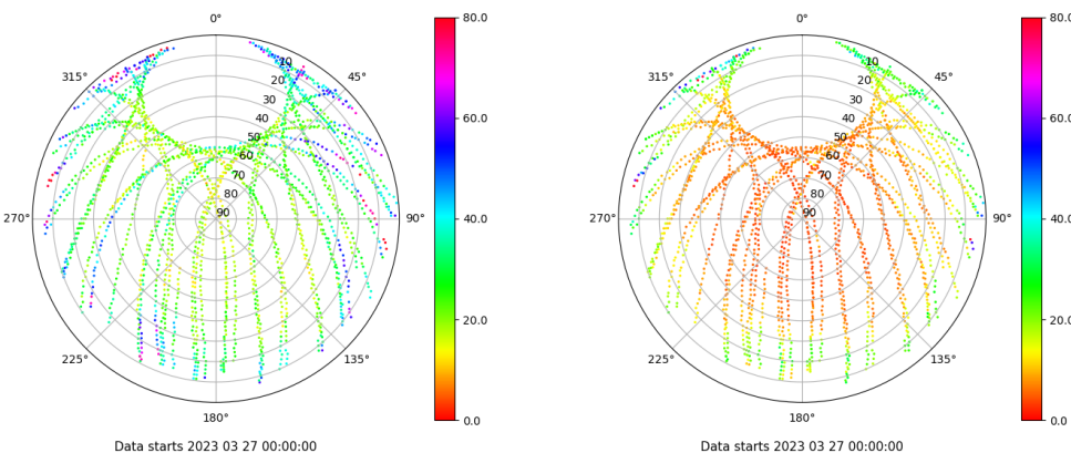
Skyplot for station SPAB. Parameter M1C Data file SPAB00ESP_R_2023086.xtr Skyplot for station SPAB. Parameter M2P Data file SPAB00ESP_R_2023086.xtr
