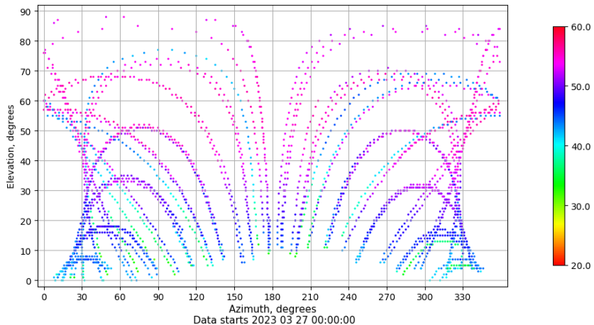
Azimuth-elevation plot for station SPAB. Signal to Noise S1C Data file SPAB00ESP_R_2023086.xtr
