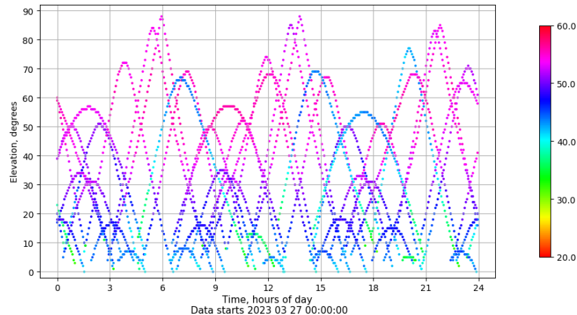
Time-elevation plot for station SPAB. Signal to Noise S1C Data file SPAB00ESP_R_2023086.xtr
