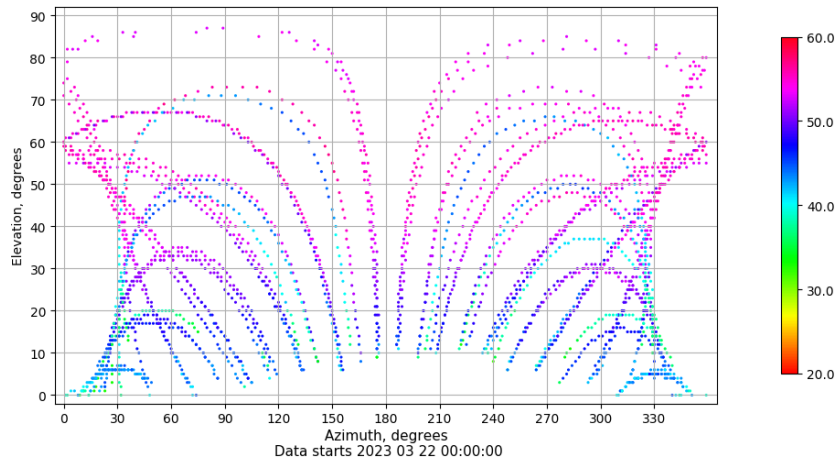
Azimuth-elevation plot for station SPAB. Signal to Noise S1C Data file SPAB00ESP_R_2023081.xtr
