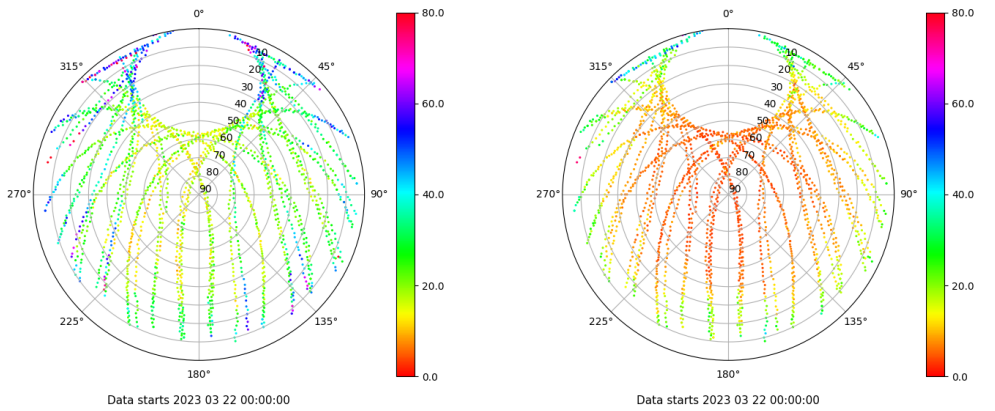
Skyplot for station SPAB. Parameter M1C Data file SPAB00ESP_R_2023081.xtr Skyplot for station SPAB. Parameter M2P Data file SPAB00ESP_R_2023081.xtr
