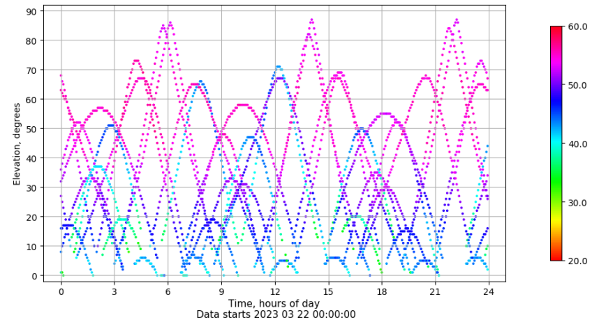
Time-elevation plot for station SPAB. Signal to Noise S1C Data file SPAB00ESP_R_2023081.xtr
