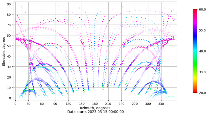
Azimuth-elevation plot for station SPAB. Signal to Noise S1C Data file SPAB00ESP_R_2023074.xtr
