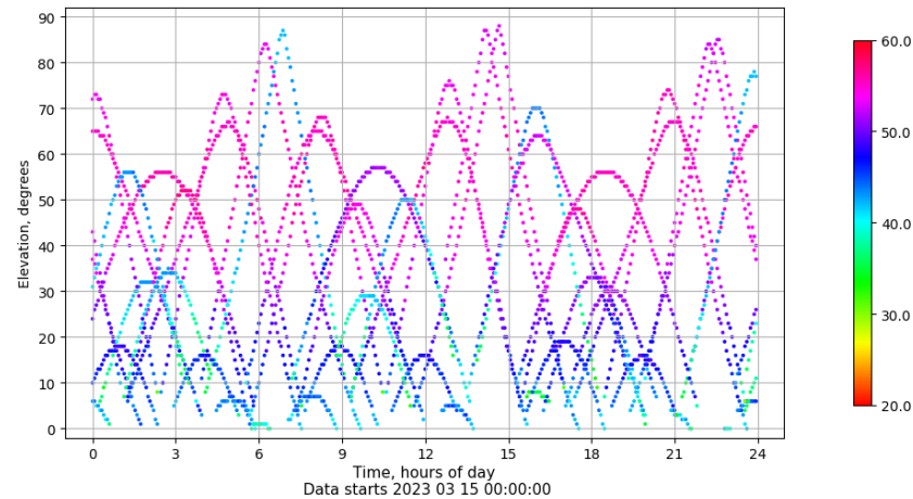
Time-elevation plot for station SPAB. Signal to Noise S1C Data file SPAB00ESP_R_2023074.xtr
