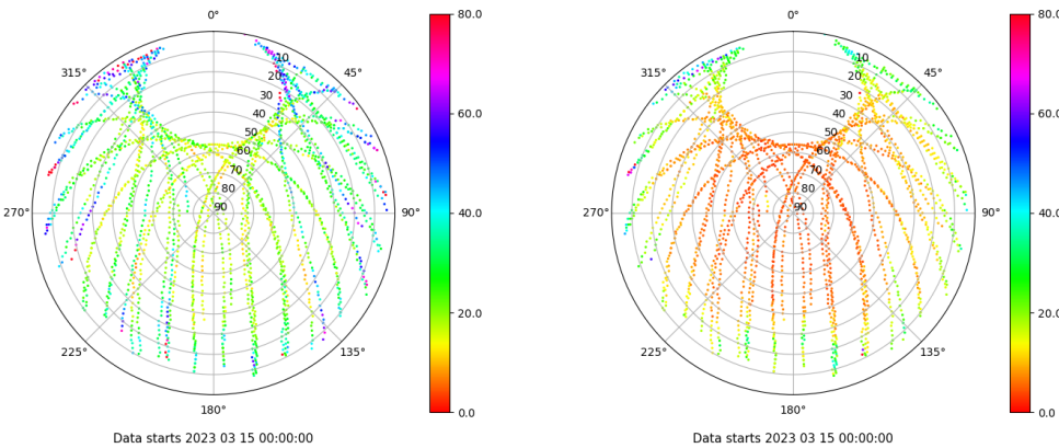
Skyplot for station SPAB. Parameter M1C Data file SPAB00ESP_R_2023074.xtr Skyplot for station SPAB. Parameter M2P Data file SPAB00ESP_R_2023074.xtr
