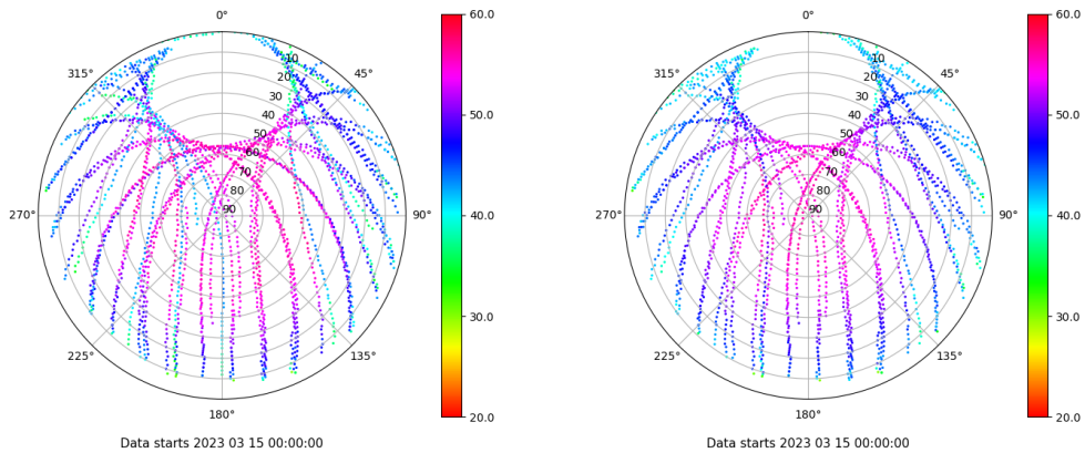
Skyplot for station SPAB. Signal to Noise S1C Data file SPAB00ESP_R_2023074.xtr Skyplot for station SPAB. Signal to Noise S2P Data file SPAB00ESP_R_2023074.xtr
