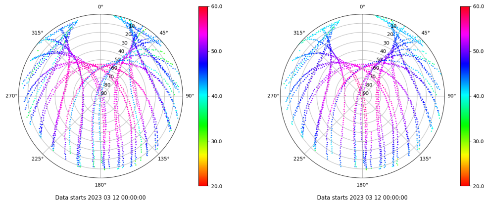
Skyplot for station SPAB. Signal to Noise S1C Data file SPAB00ESP_R_2023071.xtr Skyplot for station SPAB. Signal to Noise S2P Data file SPAB00ESP_R_2023071.xtr
