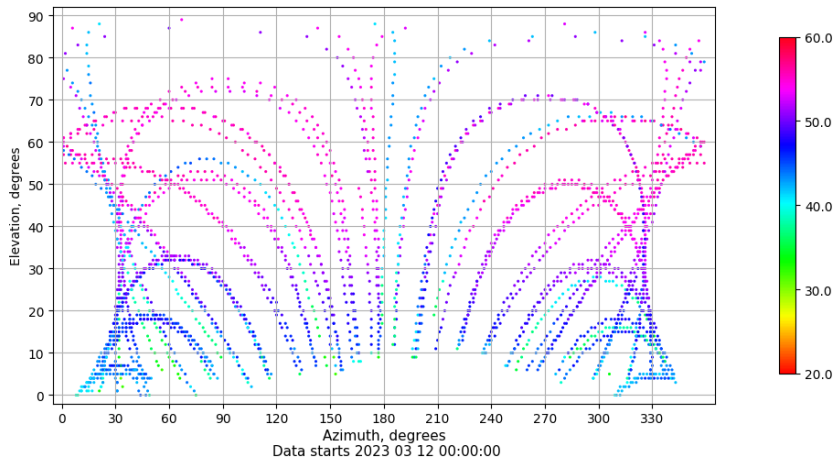
Azimuth-elevation plot for station SPAB. Signal to Noise S1C Data file SPAB00ESP_R_2023071.xtr
