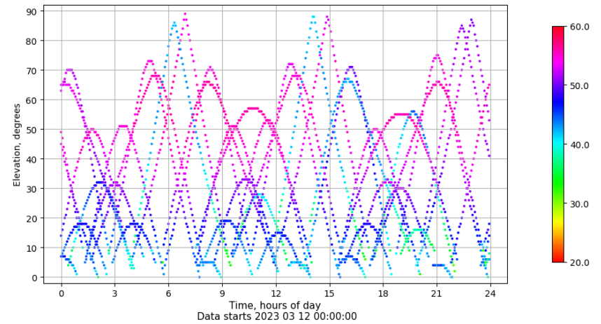
Time-elevation plot for station SPAB. Signal to Noise S1C Data file SPAB00ESP_R_2023071.xtr
