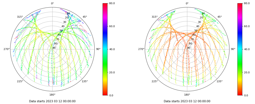
Skyplot for station SPAB. Parameter M1C Data file SPAB00ESP_R_2023071.xtr Skyplot for station SPAB. Parameter M2P Data file SPAB00ESP_R_2023071.xtr
