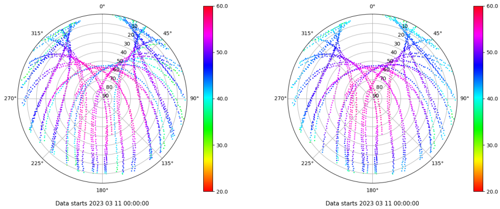
Skyplot for station SPAB. Signal to Noise S1C Data file SPAB00ESP_R_2023070.xtr Skyplot for station SPAB. Signal to Noise S2P Data file SPAB00ESP_R_2023070.xtr
