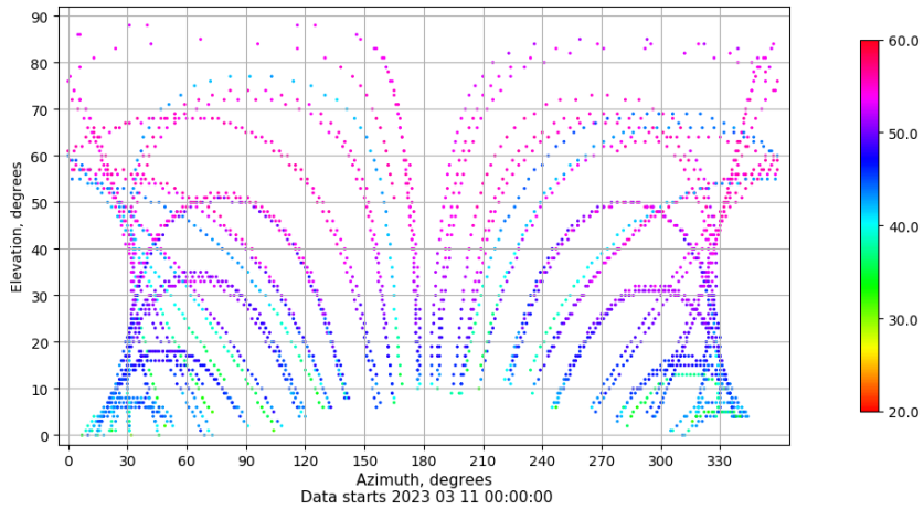
Azimuth-elevation plot for station SPAB. Signal to Noise S1C Data file SPAB00ESP_R_2023070.xtr
