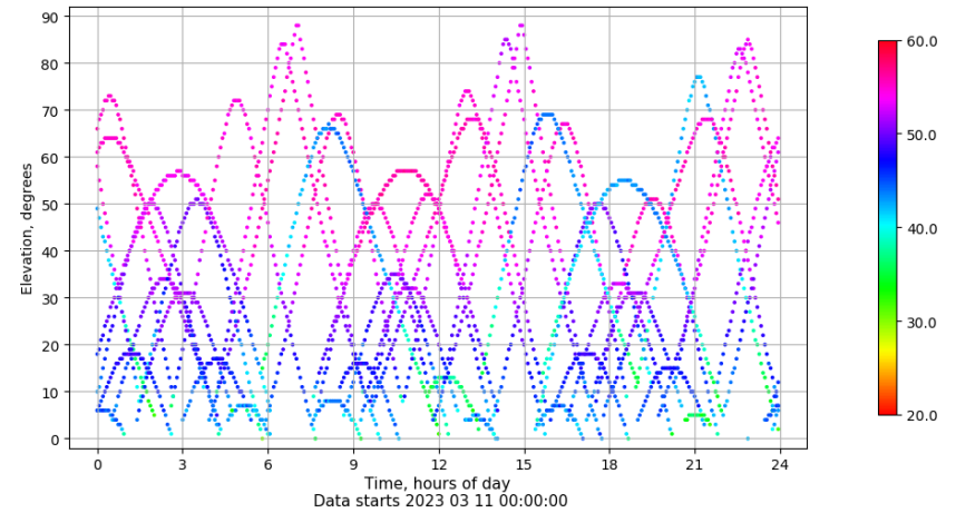
Time-elevation plot for station SPAB. Signal to Noise S1C Data file SPAB00ESP_R_2023070.xtr
