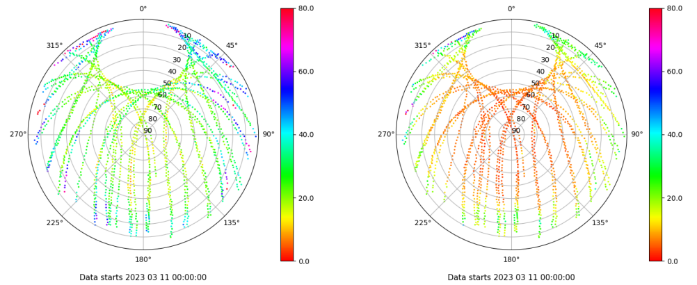
Skyplot for station SPAB. Parameter M1C Data file SPAB00ESP_R_2023070.xtr Skyplot for station SPAB. Parameter M2P Data file SPAB00ESP_R_2023070.xtr
